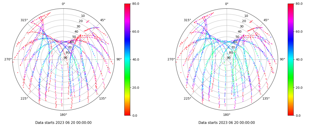
Skyplot for station ALC1. Parameter M1C Data file ALC100ESP_R_2023171.xtr Skyplot for station ALC1. Parameter M2C Data file ALC100ESP_R_2023171.xtr
