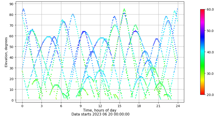
Time-elevation plot for station ALC1. Signal to Noise S1C Data file ALC100ESP_R_2023171.xtr
