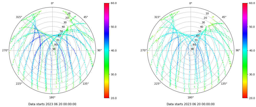
Skyplot for station ALC1. Signal to Noise S1C Data file ALC100ESP_R_2023171.xtr Skyplot for station ALC1. Signal to Noise S2C Data file ALC100ESP_R_2023171.xtr
