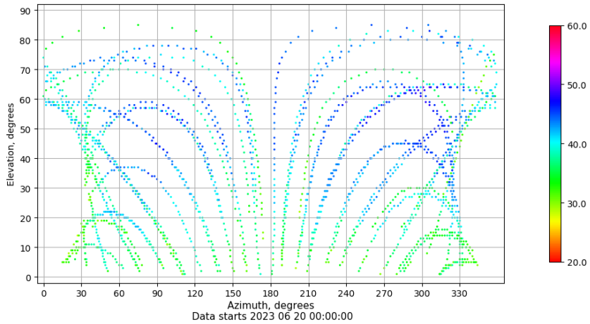
Azimuth-elevation plot for station ALC1. Signal to Noise S1C Data file ALC100ESP_R_2023171.xtr
