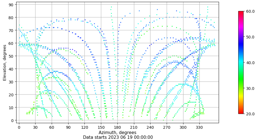
Azimuth-elevation plot for station ALC1. Signal to Noise S1C Data file ALC100ESP_R_2023170.xtr
