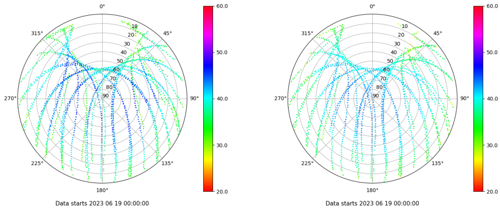
Skyplot for station ALC1. Signal to Noise S1C Data file ALC100ESP_R_2023170.xtr Skyplot for station ALC1. Signal to Noise S2C Data file ALC100ESP_R_2023170.xtr
