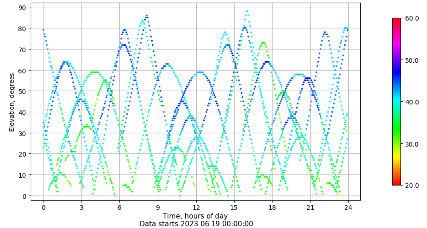
Time-elevation plot for station ALC1. Signal to Noise S1C Data file ALC100ESP_R_2023170.xtr
