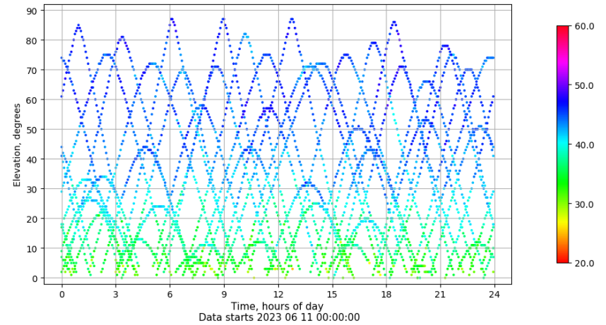
Time-elevation plot for station ALC1. Signal to Noise S1C Data file ALC100ESP_R_2023162.xtr
