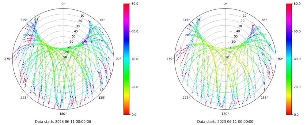
Skyplot for station ALC1. Parameter M1C Data file ALC100ESP_R_2023162.xtr Skyplot for station ALC1. Parameter M2X Data file ALC100ESP_R_2023162.xtr
