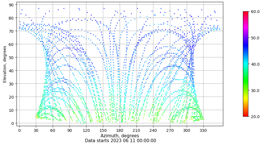
Azimuth-elevation plot for station ALC1. Signal to Noise S1C Data file ALC100ESP_R_2023162.xtr
