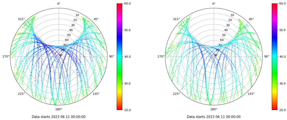
Skyplot for station ALC1. Signal to Noise S1C Data file ALC100ESP_R_2023162.xtr Skyplot for station ALC1. Signal to Noise S2X Data file ALC100ESP_R_2023162.xtr
