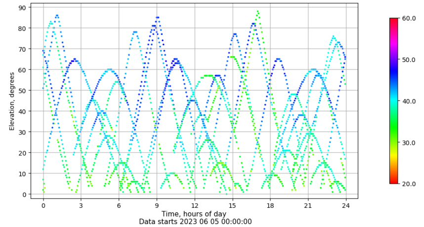
Time-elevation plot for station ALC1. Signal to Noise S1C Data file ALC100ESP_R_2023156.xtr
