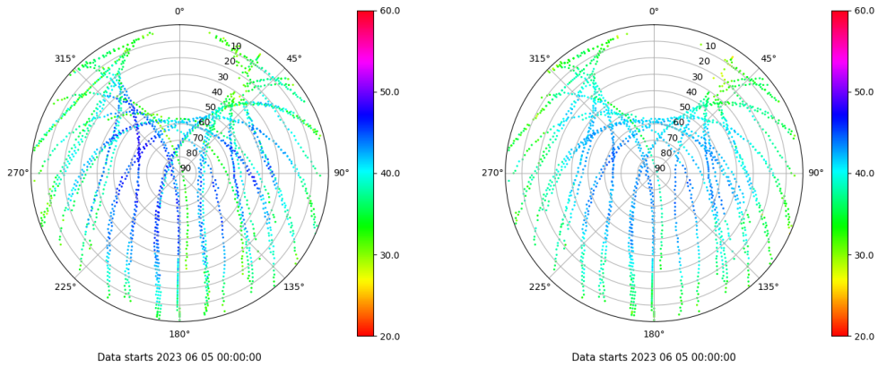
Skyplot for station ALC1. Signal to Noise S1C Data file ALC100ESP_R_2023156.xtr Skyplot for station ALC1. Signal to Noise S2C Data file ALC100ESP_R_2023156.xtr
