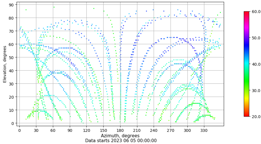
Azimuth-elevation plot for station ALC1. Signal to Noise S1C Data file ALC100ESP_R_2023156.xtr
