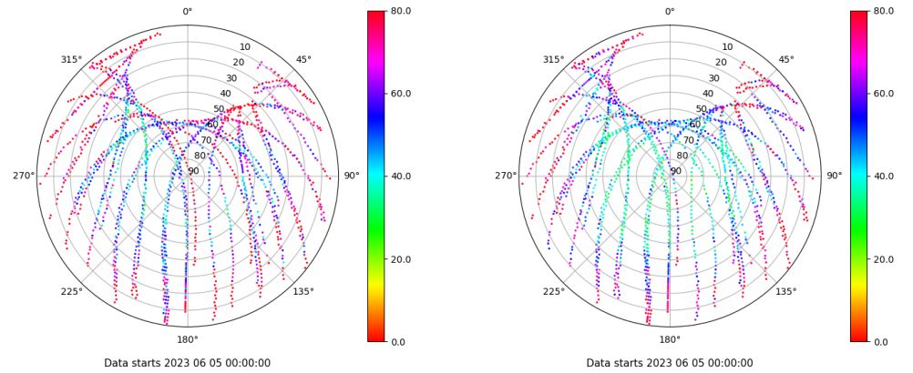
Skyplot for station ALC1. Parameter M1C Data file ALC100ESP_R_2023156.xtr Skyplot for station ALC1. Parameter M2C Data file ALC100ESP_R_2023156.xtr
