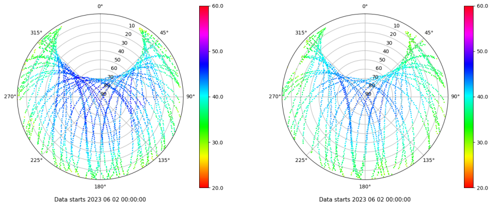
Skyplot for station ALC1. Signal to Noise S1C Data file ALC100ESP_R_2023153.xtr Skyplot for station ALC1. Signal to Noise S2X Data file ALC100ESP_R_2023153.xtr
