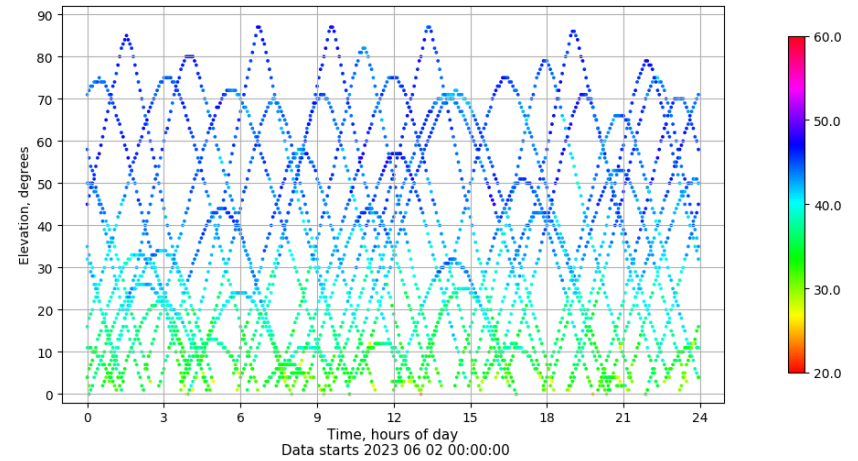
Time-elevation plot for station ALC1. Signal to Noise S1C Data file ALC100ESP_R_2023153.xtr
