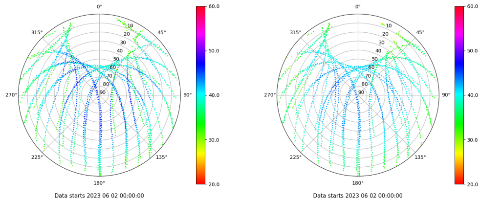
Skyplot for station ALC1. Signal to Noise S1C Data file ALC100ESP_R_2023153.xtr Skyplot for station ALC1. Signal to Noise S2C Data file ALC100ESP_R_2023153.xtr
