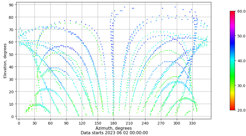
Azimuth-elevation plot for station ALC1. Signal to Noise S1C Data file ALC100ESP_R_2023153.xtr
