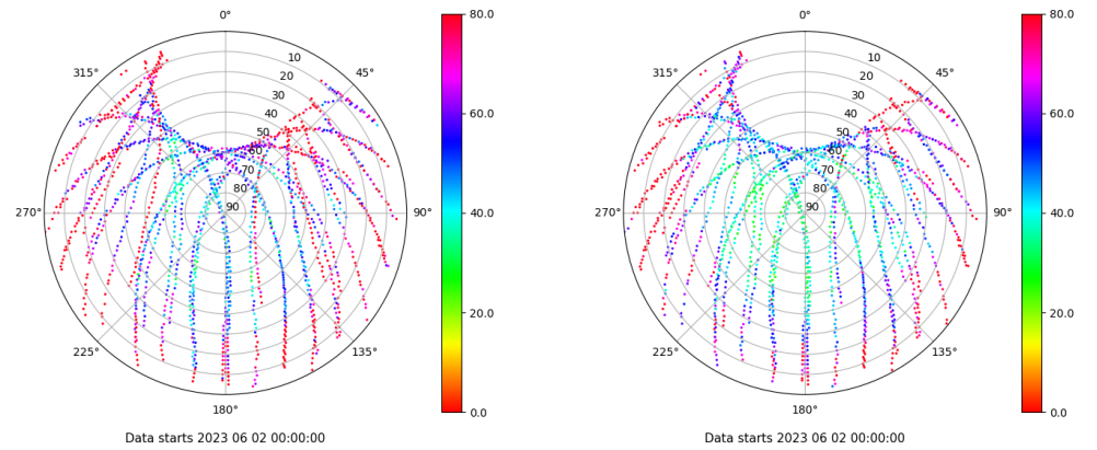
Skyplot for station ALC1. Parameter M1C Data file ALC100ESP_R_2023153.xtr Skyplot for station ALC1. Parameter M2C Data file ALC100ESP_R_2023153.xtr
