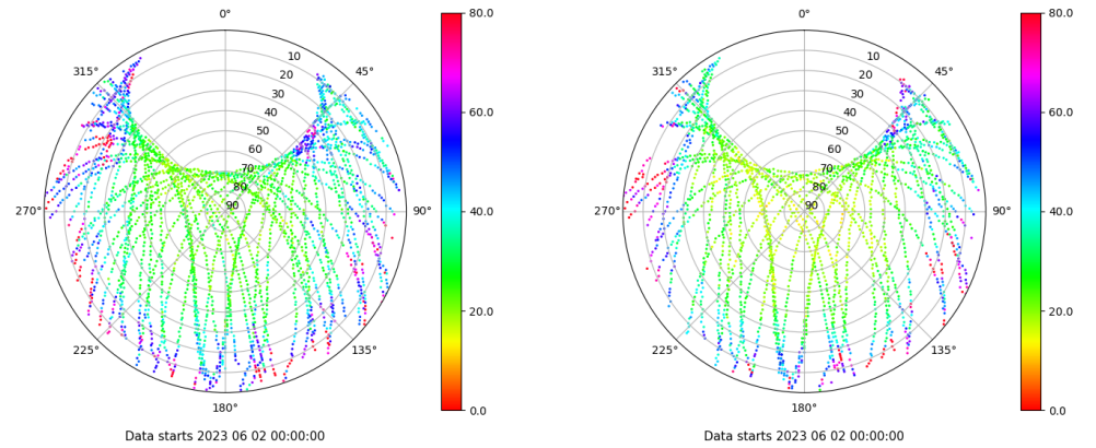
Skyplot for station ALC1. Parameter M1C Data file ALC100ESP_R_2023153.xtr Skyplot for station ALC1. Parameter M2X Data file ALC100ESP_R_2023153.xtr
