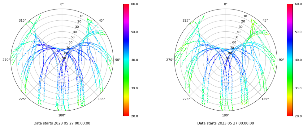
Skyplot for station ALC1. Signal to Noise S1X Data file ALC100ESP_R_2023147.xtr Skyplot for station ALC1. Signal to Noise S5X Data file ALC100ESP_R_2023147.xtr
