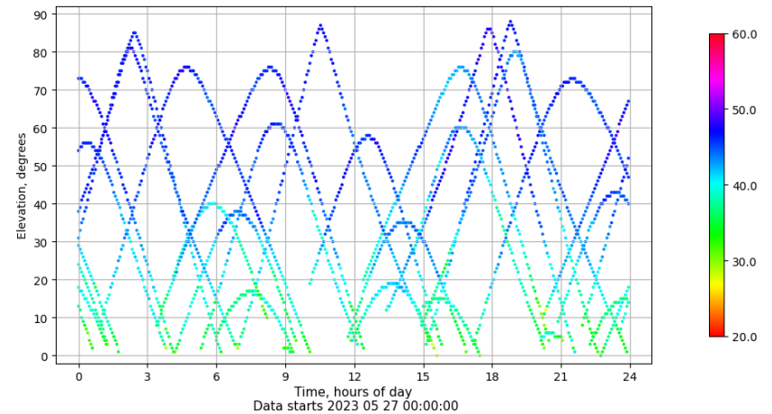
Time-elevation plot for station ALC1. Signal to Noise S1X Data file ALC100ESP_R_2023147.xtr
