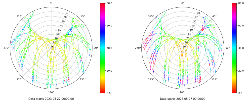
Skyplot for station ALC1. Parameter M1X Data file ALC100ESP_R_2023147.xtr Skyplot for station ALC1. Parameter M5X Data file ALC100ESP_R_2023147.xtr
