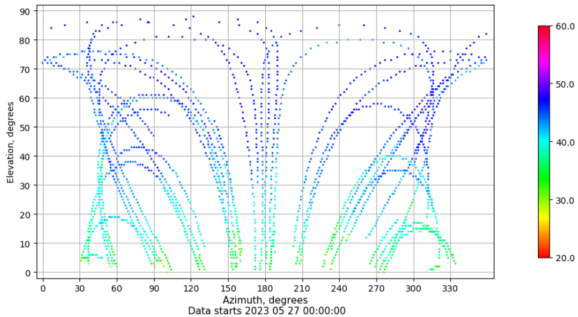
Azimuth-elevation plot for station ALC1. Signal to Noise S1X Data file ALC100ESP_R_2023147.xtr
