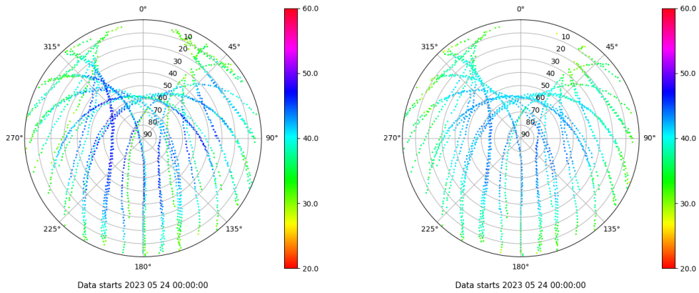
Skyplot for station ALC1. Signal to Noise S1C Data file ALC100ESP_R_2023144.xtr Skyplot for station ALC1. Signal to Noise S2C Data file ALC100ESP_R_2023144.xtr
