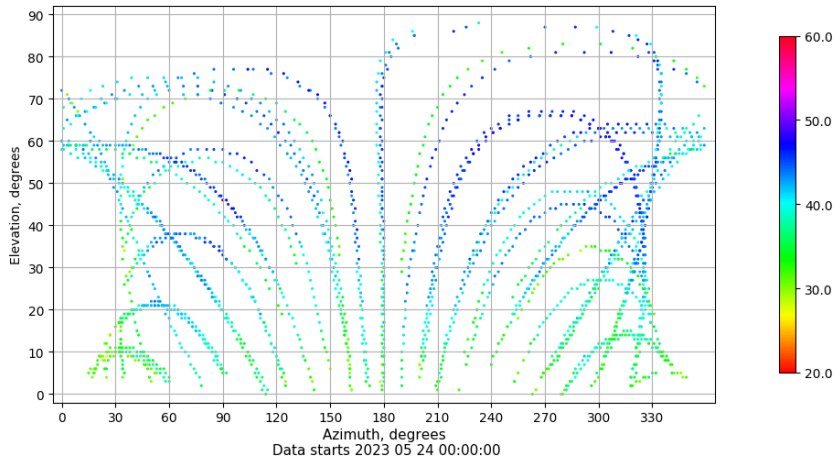
Azimuth-elevation plot for station ALC1. Signal to Noise S1C Data file ALC100ESP_R_2023144.xtr
