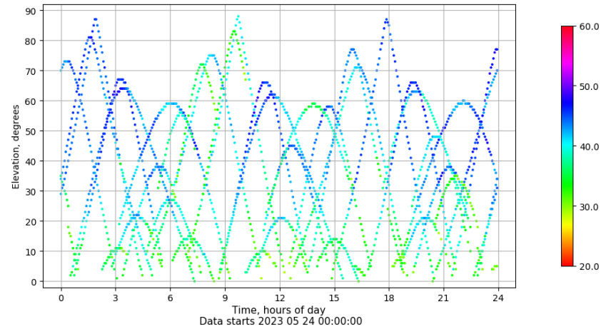
Time-elevation plot for station ALC1. Signal to Noise S1C Data file ALC100ESP_R_2023144.xtr
