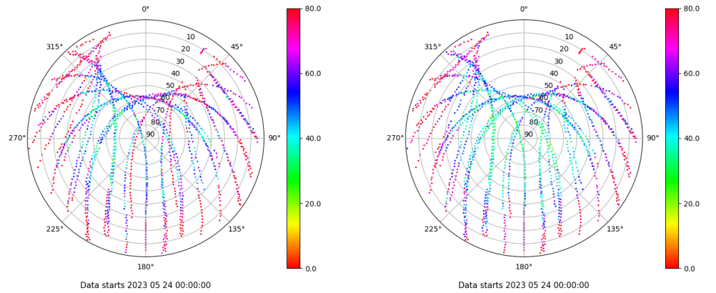
Skyplot for station ALC1. Parameter M1C Data file ALC100ESP_R_2023144.xtr Skyplot for station ALC1. Parameter M2C Data file ALC100ESP_R_2023144.xtr
