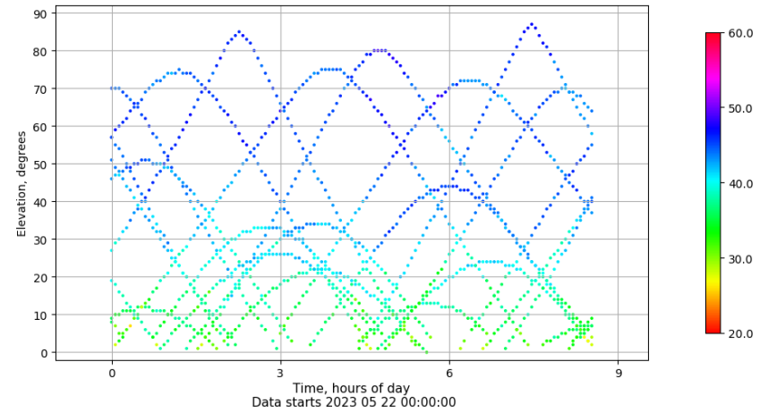
Time-elevation plot for station ALC1. Signal to Noise S1C Data file ALC100ESP_R_2023142.xtr
