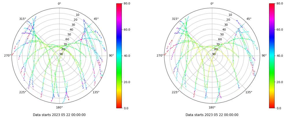
Skyplot for station ALC1. Parameter M1C Data file ALC100ESP_R_2023142.xtr Skyplot for station ALC1. Parameter M2X Data file ALC100ESP_R_2023142.xtr
