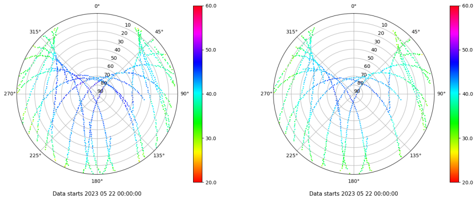
Skyplot for station ALC1. Signal to Noise S1C Data file ALC100ESP_R_2023142.xtr Skyplot for station ALC1. Signal to Noise S2X Data file ALC100ESP_R_2023142.xtr
