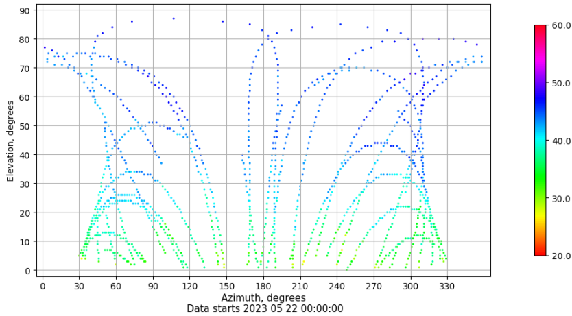
Azimuth-elevation plot for station ALC1. Signal to Noise S1C Data file ALC100ESP_R_2023142.xtr
