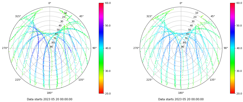
Skyplot for station ALC1. Signal to Noise S1C Data file ALC100ESP_R_2023140.xtr Skyplot for station ALC1. Signal to Noise S2C Data file ALC100ESP_R_2023140.xtr
