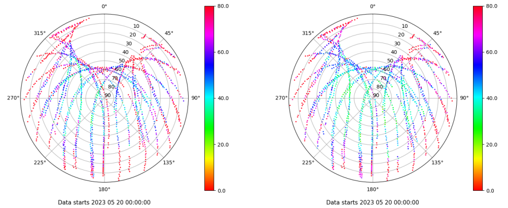
Skyplot for station ALC1. Parameter M1C Data file ALC100ESP_R_2023140.xtr Skyplot for station ALC1. Parameter M2C Data file ALC100ESP_R_2023140.xtr
