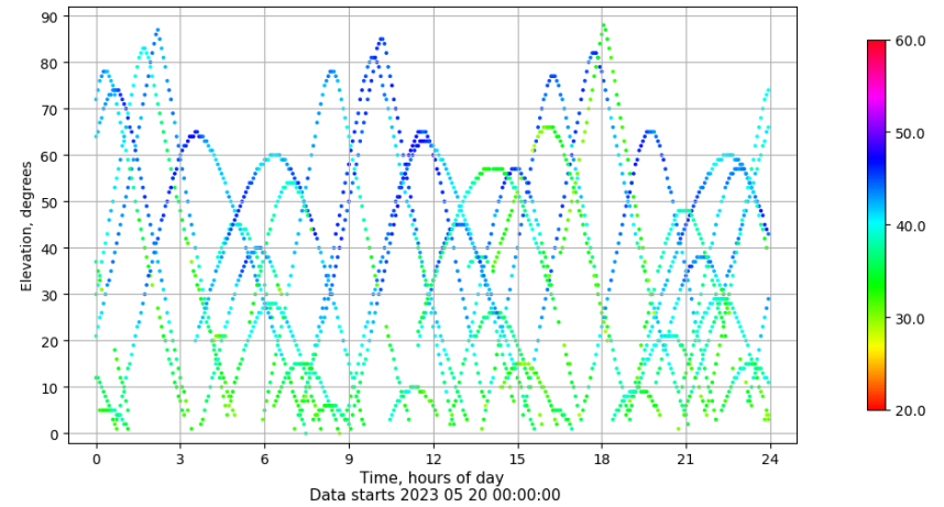
Time-elevation plot for station ALC1. Signal to Noise S1C Data file ALC100ESP_R_2023140.xtr
