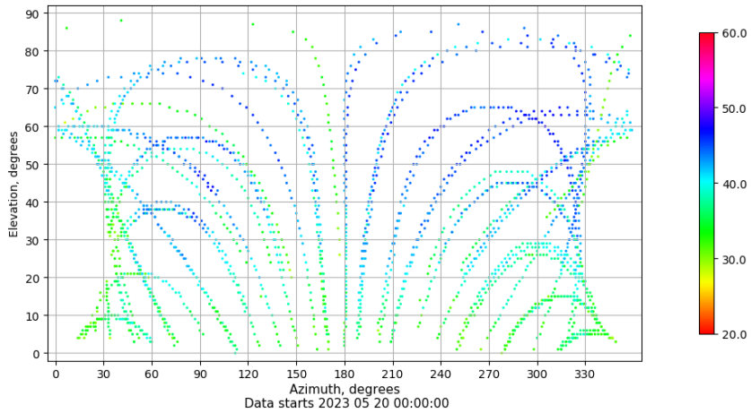
Azimuth-elevation plot for station ALC1. Signal to Noise S1C Data file ALC100ESP_R_2023140.xtr
