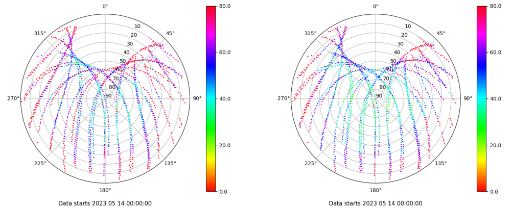
Skyplot for station ALC1. Parameter M1C Data file ALC100ESP_R_2023134.xtr Skyplot for station ALC1. Parameter M2C Data file ALC100ESP_R_2023134.xtr
