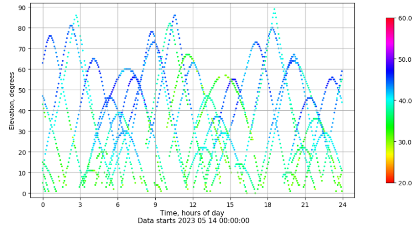
Time-elevation plot for station ALC1. Signal to Noise S1C Data file ALC100ESP_R_2023134.xtr
