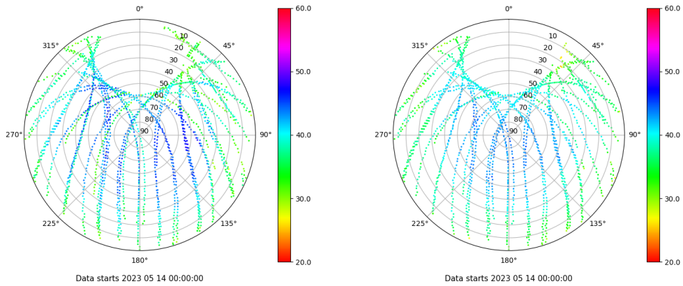
Skyplot for station ALC1. Signal to Noise S1C Data file ALC100ESP_R_2023134.xtr Skyplot for station ALC1. Signal to Noise S2C Data file ALC100ESP_R_2023134.xtr
