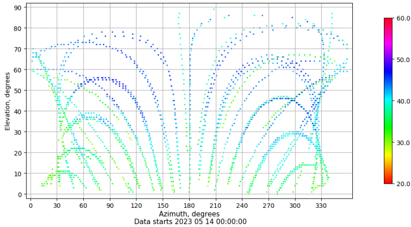
Azimuth-elevation plot for station ALC1. Signal to Noise S1C Data file ALC100ESP_R_2023134.xtr
