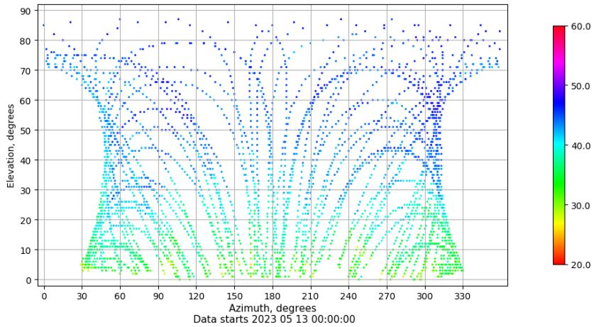
Azimuth-elevation plot for station ALC1. Signal to Noise S1C Data file ALC100ESP_R_2023133.xtr
