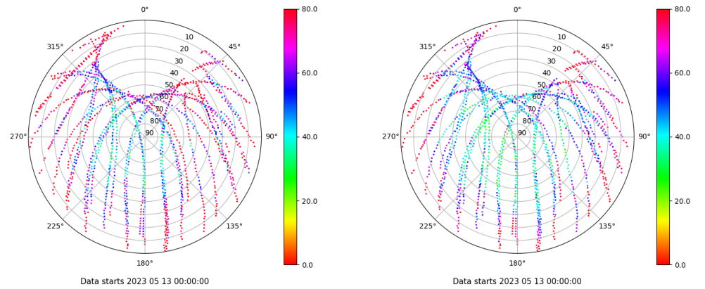
Skyplot for station ALC1. Parameter M1C Data file ALC100ESP_R_2023133.xtr Skyplot for station ALC1. Parameter M2C Data file ALC100ESP_R_2023133.xtr
