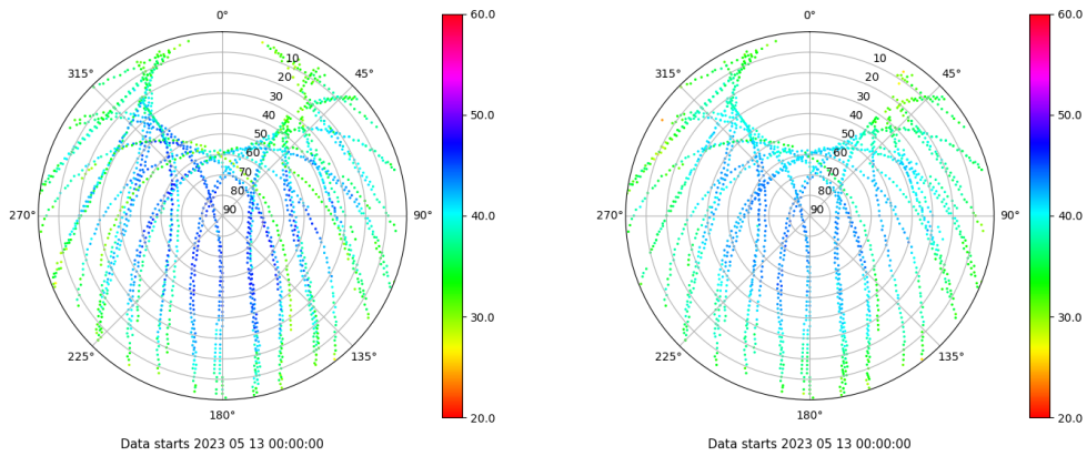
Skyplot for station ALC1. Signal to Noise S1C Data file ALC100ESP_R_2023133.xtr Skyplot for station ALC1. Signal to Noise S2C Data file ALC100ESP_R_2023133.xtr
