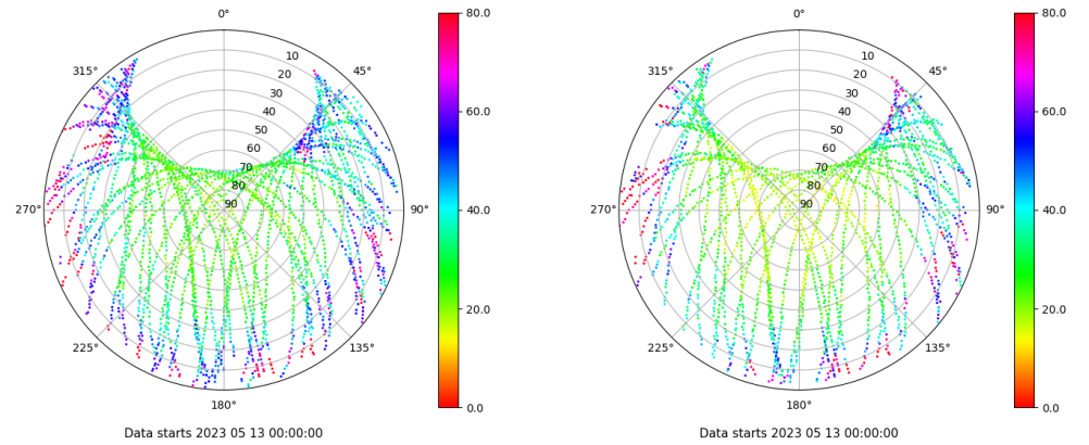
Skyplot for station ALC1. Parameter M1C Data file ALC100ESP_R_2023133.xtr Skyplot for station ALC1. Parameter M2X Data file ALC100ESP_R_2023133.xtr
