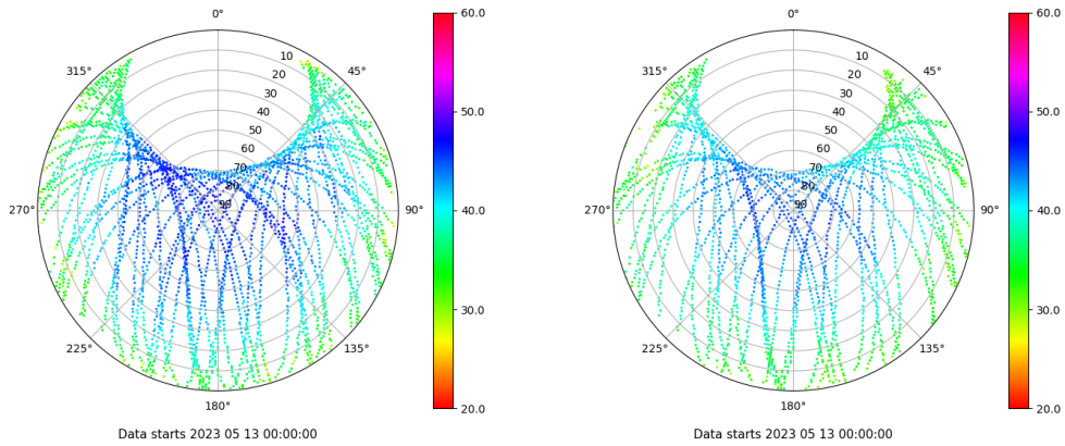
Skyplot for station ALC1. Signal to Noise S1C Data file ALC100ESP_R_2023133.xtr Skyplot for station ALC1. Signal to Noise S2X Data file ALC100ESP_R_2023133.xtr
