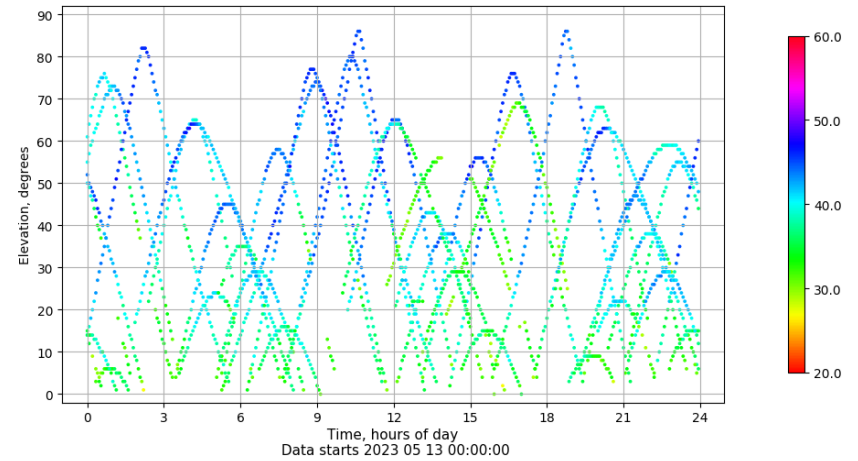
Time-elevation plot for station ALC1. Signal to Noise S1C Data file ALC100ESP_R_2023133.xtr
