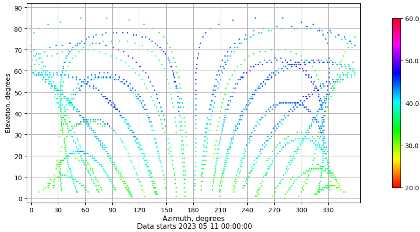
Azimuth-elevation plot for station ALC1. Signal to Noise S1C Data file ALC100ESP_R_2023131.xtr
