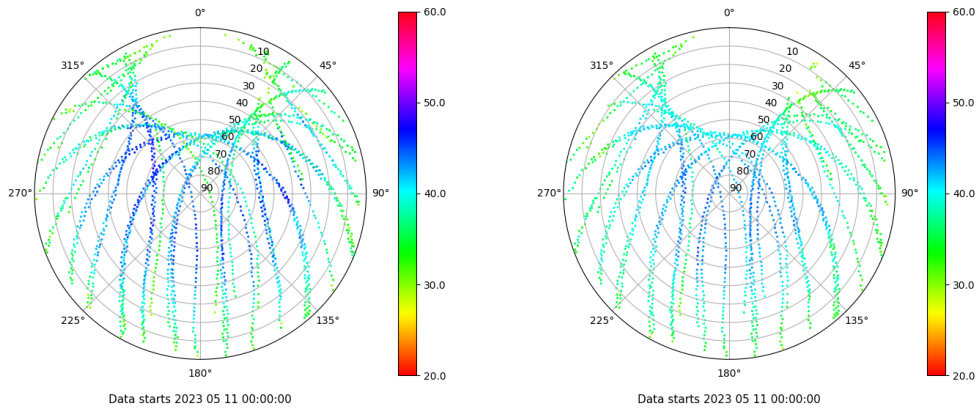
Skyplot for station ALC1. Signal to Noise S1C Data file ALC100ESP_R_2023131.xtr Skyplot for station ALC1. Signal to Noise S2C Data file ALC100ESP_R_2023131.xtr
