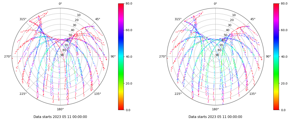
Skyplot for station ALC1. Parameter M1C Data file ALC100ESP_R_2023131.xtr Skyplot for station ALC1. Parameter M2C Data file ALC100ESP_R_2023131.xtr
