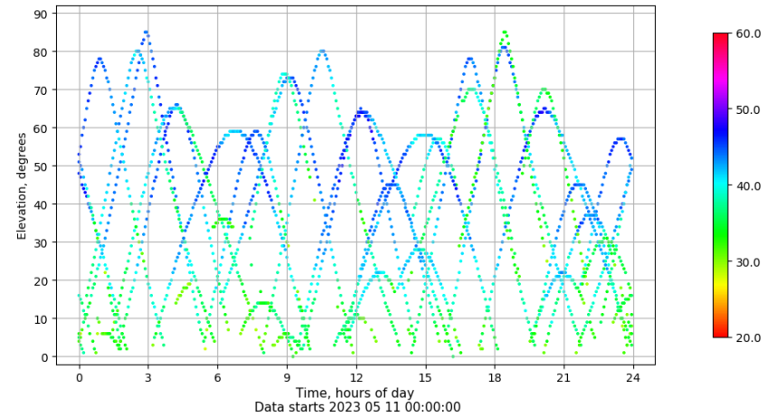
Time-elevation plot for station ALC1. Signal to Noise S1C Data file ALC100ESP_R_2023131.xtr
