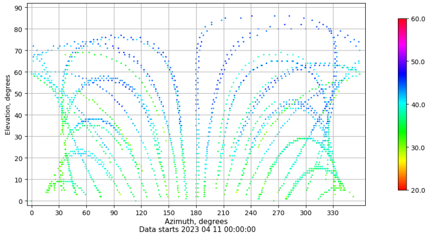
Azimuth-elevation plot for station ALC1. Signal to Noise S1C Data file ALC100ESP_R_2023101.xtr
