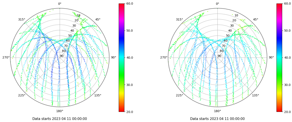
Skyplot for station ALC1. Signal to Noise S1C Data file ALC100ESP_R_2023101.xtr Skyplot for station ALC1. Signal to Noise S2C Data file ALC100ESP_R_2023101.xtr
