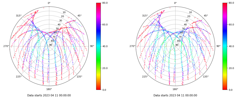
Skyplot for station ALC1. Parameter M1C Data file ALC100ESP_R_2023101.xtr Skyplot for station ALC1. Parameter M2C Data file ALC100ESP_R_2023101.xtr
