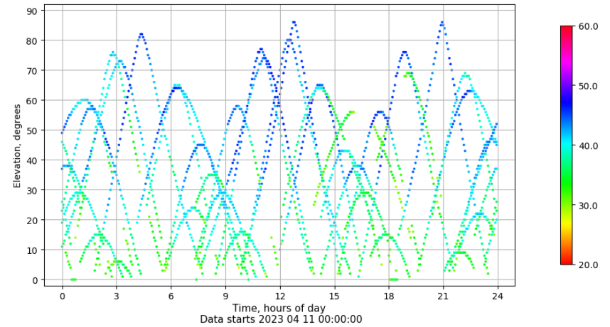
Time-elevation plot for station ALC1. Signal to Noise S1C Data file ALC100ESP_R_2023101.xtr
