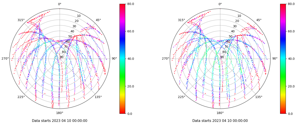
Skyplot for station ALC1. Parameter M1C Data file ALC100ESP_R_2023100.xtr Skyplot for station ALC1. Parameter M2C Data file ALC100ESP_R_2023100.xtr
