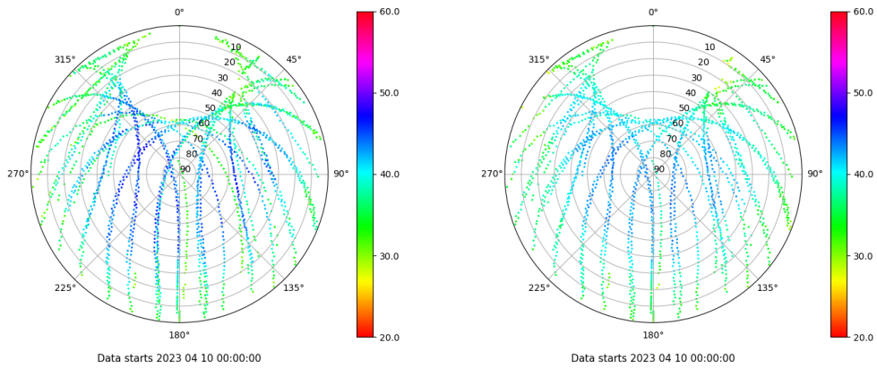
Skyplot for station ALC1. Signal to Noise S1C Data file ALC100ESP_R_2023100.xtr Skyplot for station ALC1. Signal to Noise S2C Data file ALC100ESP_R_2023100.xtr
