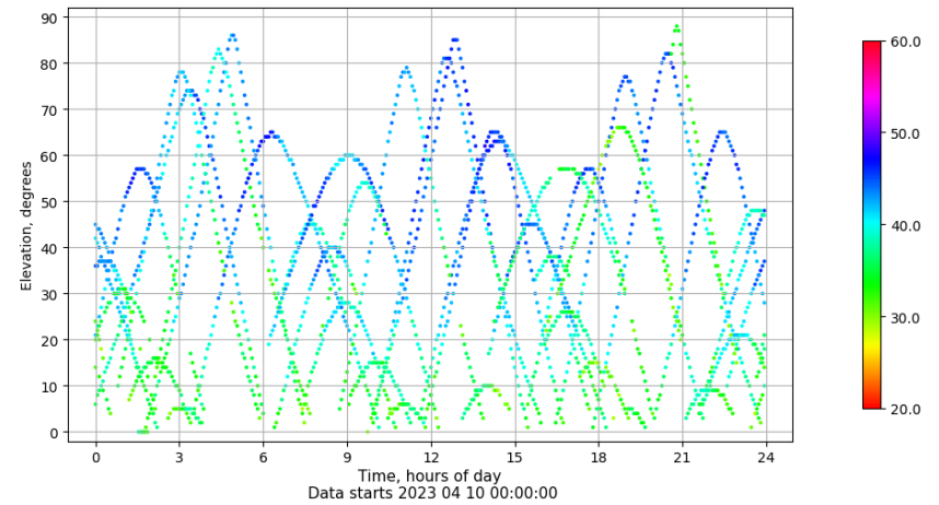
Time-elevation plot for station ALC1. Signal to Noise S1C Data file ALC100ESP_R_2023100.xtr
