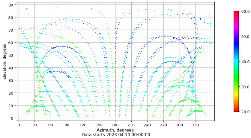
Azimuth-elevation plot for station ALC1. Signal to Noise S1C Data file ALC100ESP_R_2023100.xtr
