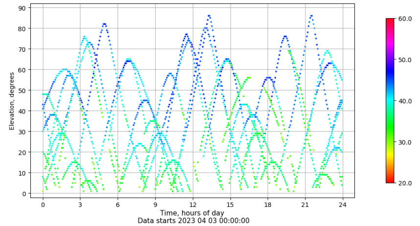
Time-elevation plot for station ALC1. Signal to Noise S1C Data file ALC100ESP_R_2023093.xtr
