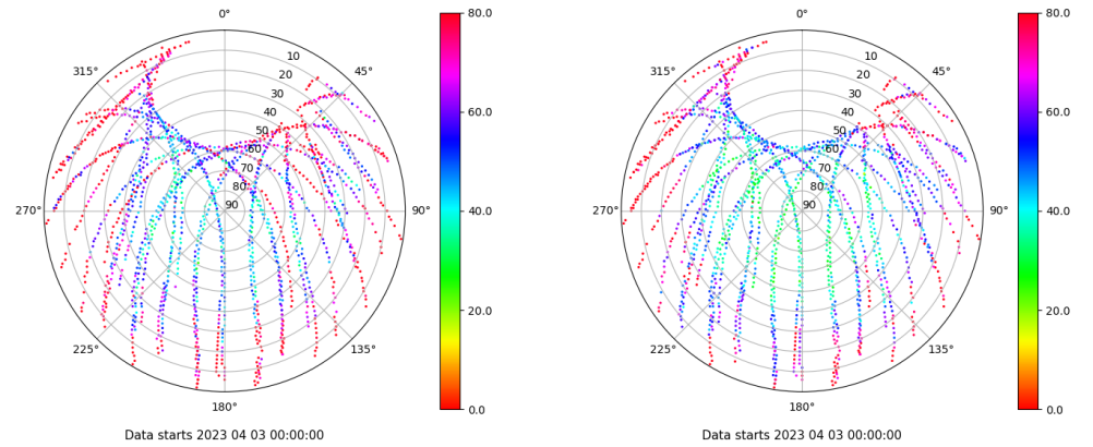
Skyplot for station ALC1. Parameter M1C Data file ALC100ESP_R_2023093.xtr Skyplot for station ALC1. Parameter M2C Data file ALC100ESP_R_2023093.xtr
