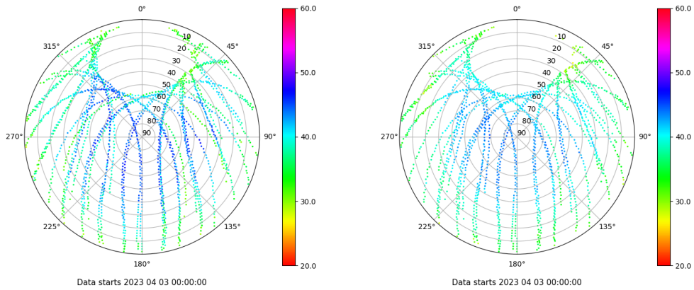
Skyplot for station ALC1. Signal to Noise S1C Data file ALC100ESP_R_2023093.xtr Skyplot for station ALC1. Signal to Noise S2C Data file ALC100ESP_R_2023093.xtr
