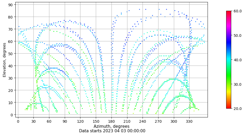
Azimuth-elevation plot for station ALC1. Signal to Noise S1C Data file ALC100ESP_R_2023093.xtr
