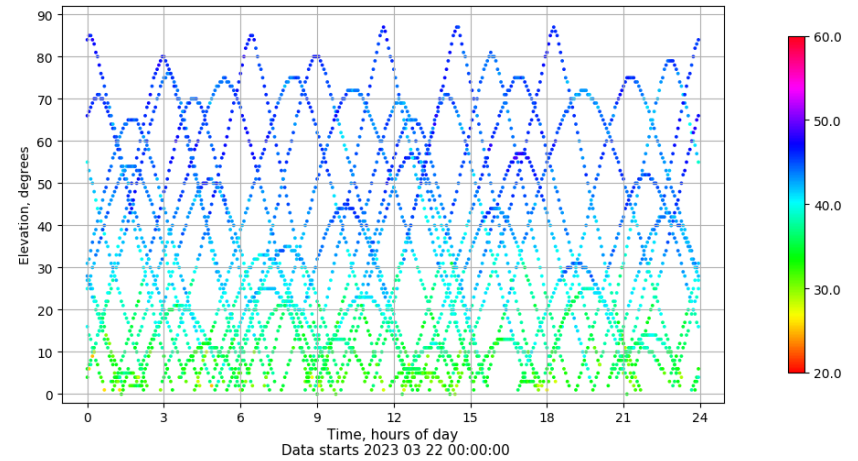
Time-elevation plot for station ALC1. Signal to Noise S1C Data file ALC100ESP_R_2023081.xtr
