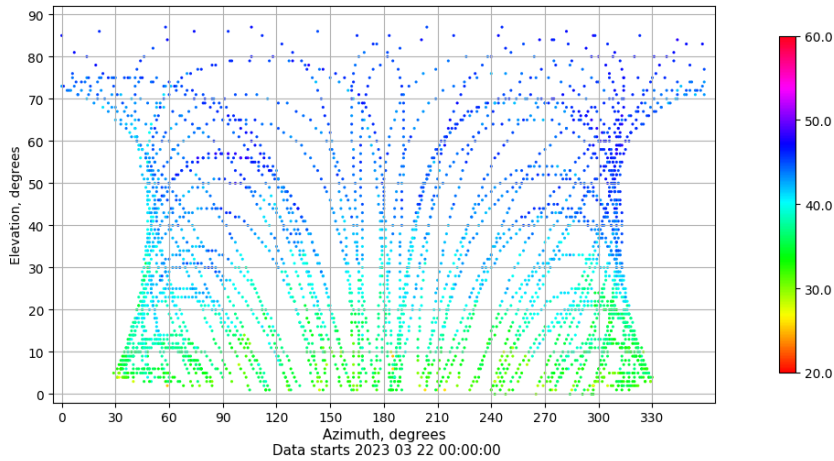
Azimuth-elevation plot for station ALC1. Signal to Noise S1C Data file ALC100ESP_R_2023081.xtr
