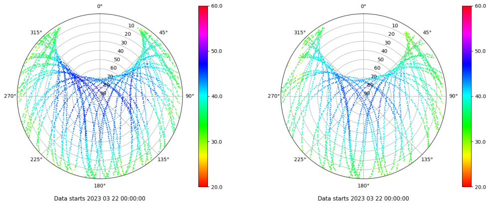
Skyplot for station ALC1. Signal to Noise S1C Data file ALC100ESP_R_2023081.xtr Skyplot for station ALC1. Signal to Noise S2X Data file ALC100ESP_R_2023081.xtr
