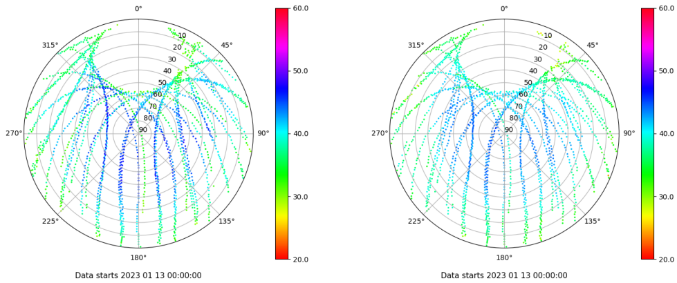
Skyplot for station ALC1. Signal to Noise S1C Data file ALC100ESP_R_2023013.xtr Skyplot for station ALC1. Signal to Noise S2C Data file ALC100ESP_R_2023013.xtr
