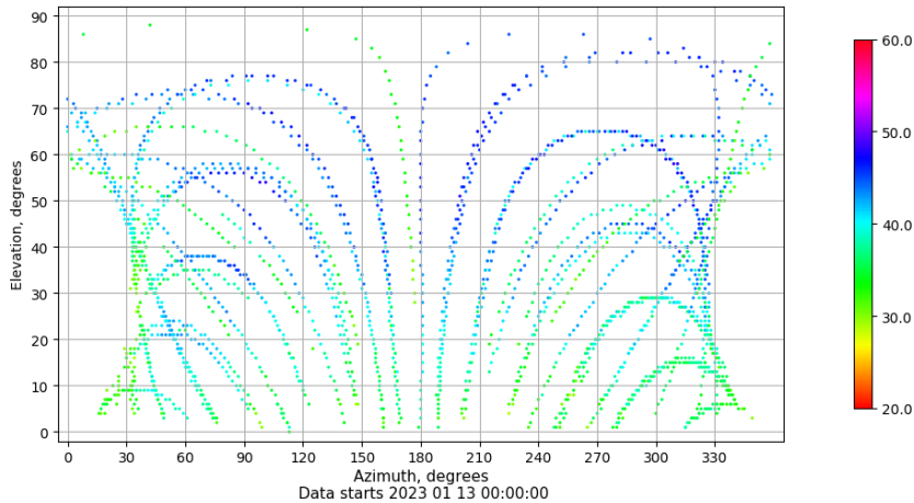
Azimuth-elevation plot for station ALC1. Signal to Noise S1C Data file ALC100ESP_R_2023013.xtr
