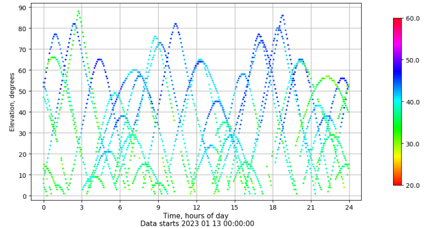
Time-elevation plot for station ALC1. Signal to Noise S1C Data file ALC100ESP_R_2023013.xtr
