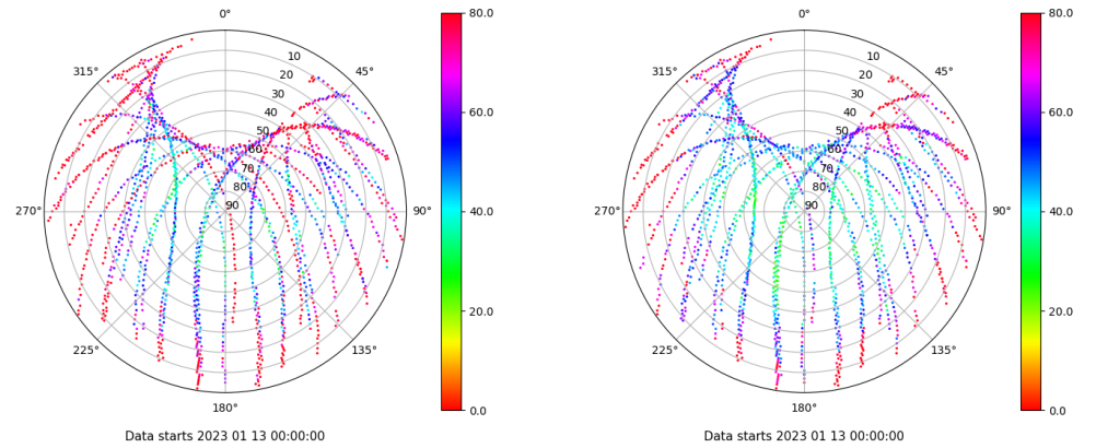
Skyplot for station ALC1. Parameter M1C Data file ALC100ESP_R_2023013.xtr Skyplot for station ALC1. Parameter M2C Data file ALC100ESP_R_2023013.xtr
