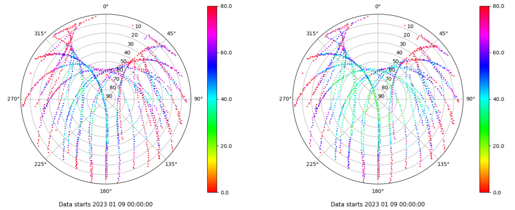
Skyplot for station ALC1. Parameter M1C Data file ALC100ESP_R_2023009.xtr Skyplot for station ALC1. Parameter M2C Data file ALC100ESP_R_2023009.xtr
