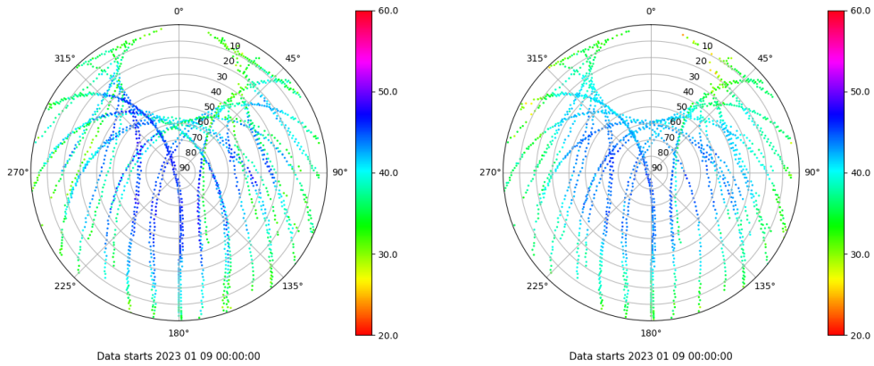
Skyplot for station ALC1. Signal to Noise S1C Data file ALC100ESP_R_2023009.xtr Skyplot for station ALC1. Signal to Noise S2C Data file ALC100ESP_R_2023009.xtr
