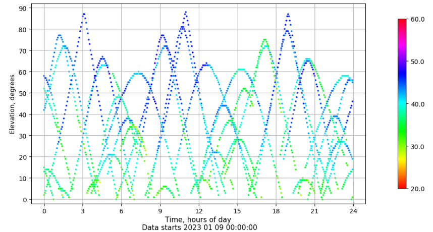
Time-elevation plot for station ALC1. Signal to Noise S1C Data file ALC100ESP_R_2023009.xtr
