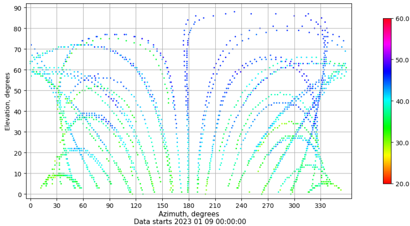
Azimuth-elevation plot for station ALC1. Signal to Noise S1C Data file ALC100ESP_R_2023009.xtr
