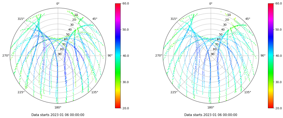
Skyplot for station ALC1. Signal to Noise S1C Data file ALC100ESP_R_2023006.xtr Skyplot for station ALC1. Signal to Noise S2C Data file ALC100ESP_R_2023006.xtr
