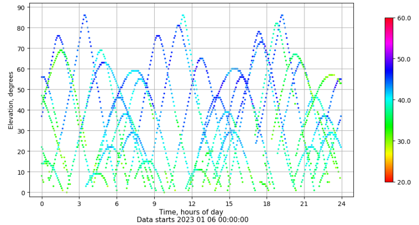
Time-elevation plot for station ALC1. Signal to Noise S1C Data file ALC100ESP_R_2023006.xtr
