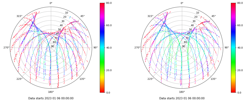
Skyplot for station ALC1. Parameter M1C Data file ALC100ESP_R_2023006.xtr Skyplot for station ALC1. Parameter M2C Data file ALC100ESP_R_2023006.xtr
