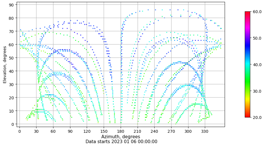
Azimuth-elevation plot for station ALC1. Signal to Noise S1C Data file ALC100ESP_R_2023006.xtr
