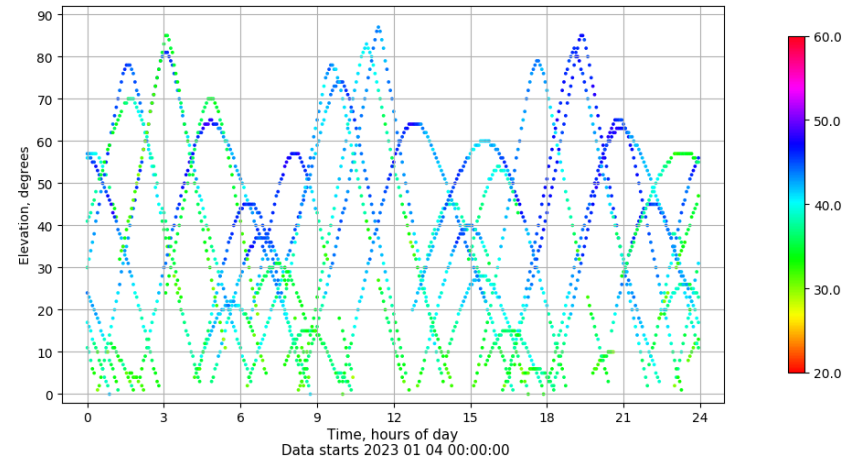
Time-elevation plot for station ALC1. Signal to Noise S1C Data file ALC100ESP_R_2023004.xtr
