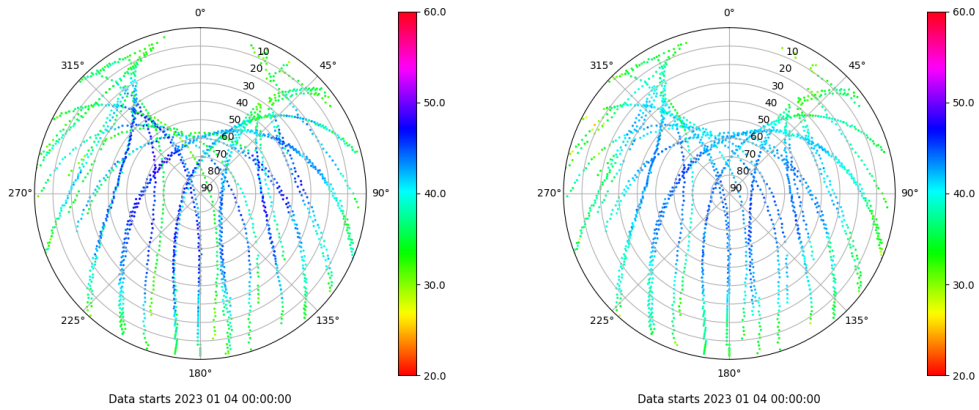
Skyplot for station ALC1. Signal to Noise S1C Data file ALC100ESP_R_2023004.xtr Skyplot for station ALC1. Signal to Noise S2C Data file ALC100ESP_R_2023004.xtr
