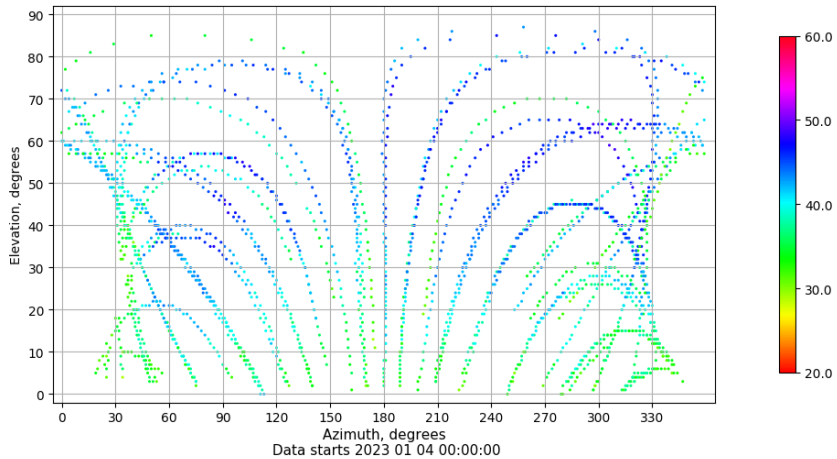
Azimuth-elevation plot for station ALC1. Signal to Noise S1C Data file ALC100ESP_R_2023004.xtr
