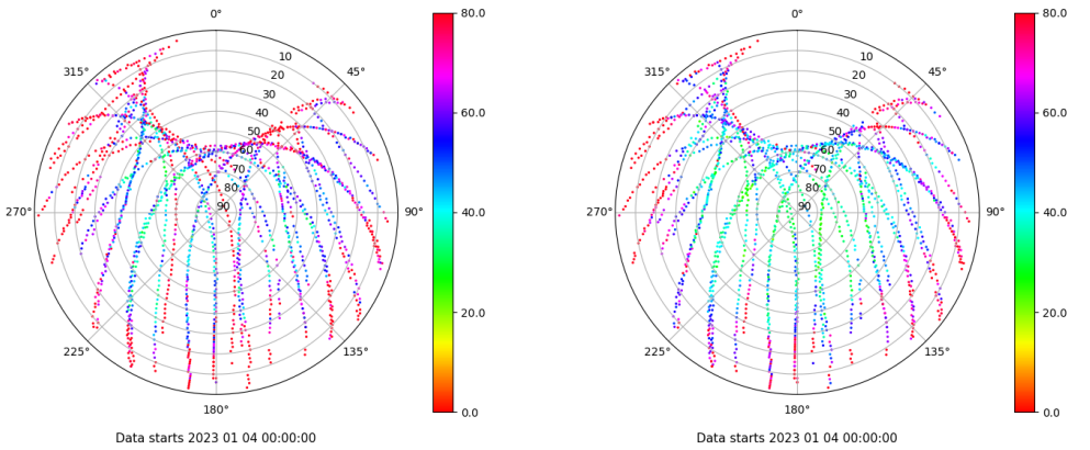
Skyplot for station ALC1. Parameter M1C Data file ALC100ESP_R_2023004.xtr Skyplot for station ALC1. Parameter M2C Data file ALC100ESP_R_2023004.xtr
