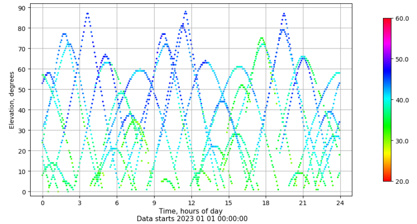
Time-elevation plot for station ALC1. Signal to Noise S1C Data file ALC100ESP_R_2023001.xtr
