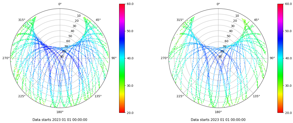
Skyplot for station ALC1. Signal to Noise S1C Data file ALC100ESP_R_2023001.xtr Skyplot for station ALC1. Signal to Noise S2X Data file ALC100ESP_R_2023001.xtr
