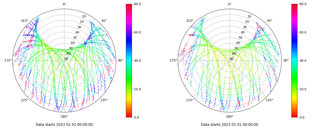
Skyplot for station ALC1. Parameter M1C Data file ALC100ESP_R_2023001.xtr Skyplot for station ALC1. Parameter M2X Data file ALC100ESP_R_2023001.xtr
