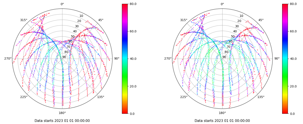
Skyplot for station ALC1. Parameter M1C Data file ALC100ESP_R_2023001.xtr Skyplot for station ALC1. Parameter M2C Data file ALC100ESP_R_2023001.xtr
