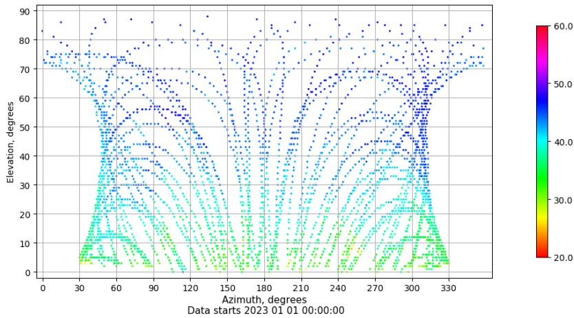
Azimuth-elevation plot for station ALC1. Signal to Noise S1C Data file ALC100ESP_R_2023001.xtr
