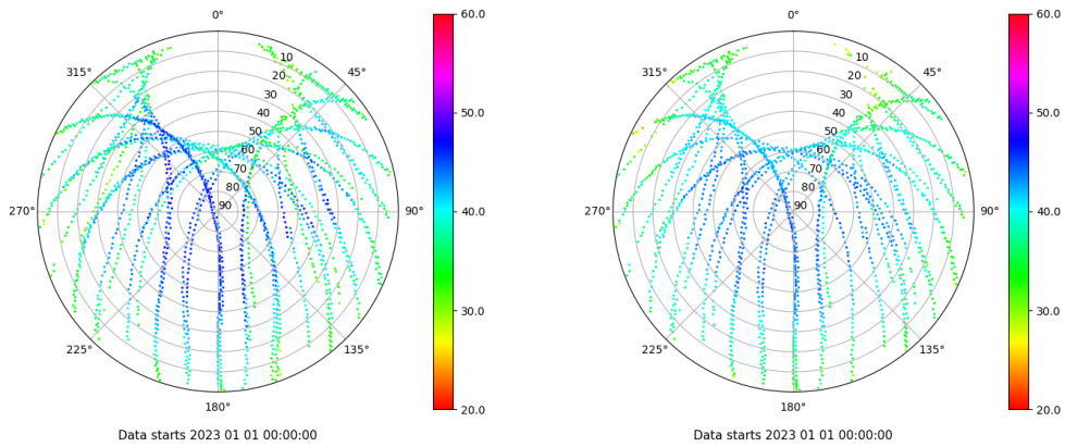
Skyplot for station ALC1. Signal to Noise S1C Data file ALC100ESP_R_2023001.xtr Skyplot for station ALC1. Signal to Noise S2C Data file ALC100ESP_R_2023001.xtr
