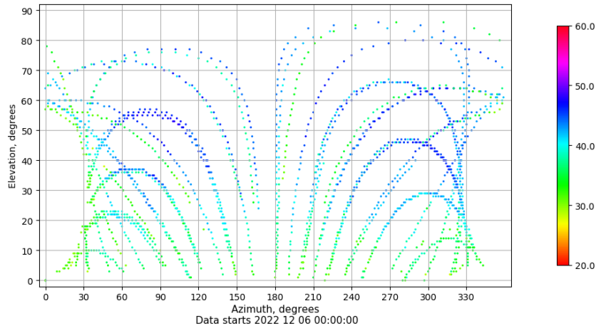
Azimuth-elevation plot for station ALC1. Signal to Noise S1C Data file ALC100ESP_R_2022340.xtr
