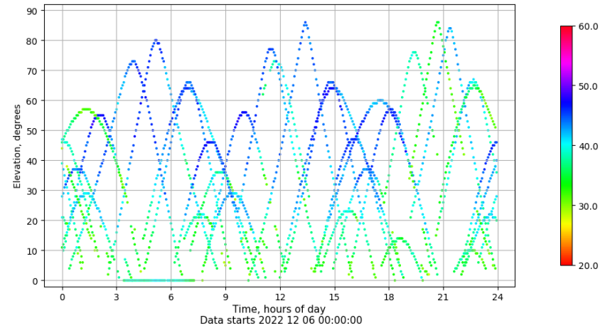
Time-elevation plot for station ALC1. Signal to Noise S1C Data file ALC100ESP_R_2022340.xtr
