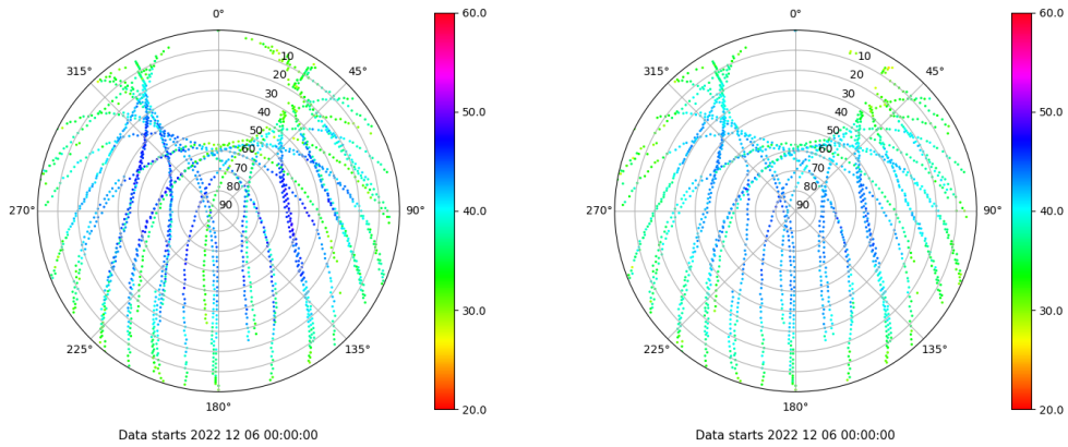
Skyplot for station ALC1. Signal to Noise S1C Data file ALC100ESP_R_2022340.xtr Skyplot for station ALC1. Signal to Noise S2C Data file ALC100ESP_R_2022340.xtr
