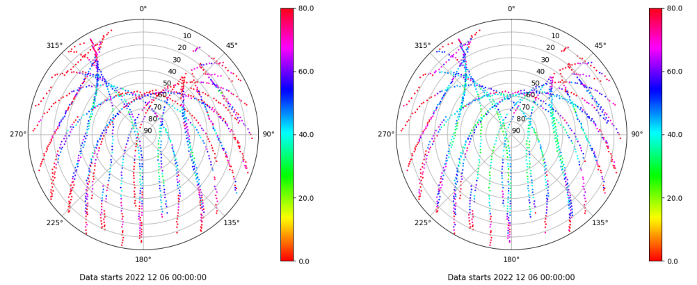
Skyplot for station ALC1. Parameter M1C Data file ALC100ESP_R_2022340.xtr Skyplot for station ALC1. Parameter M2C Data file ALC100ESP_R_2022340.xtr
