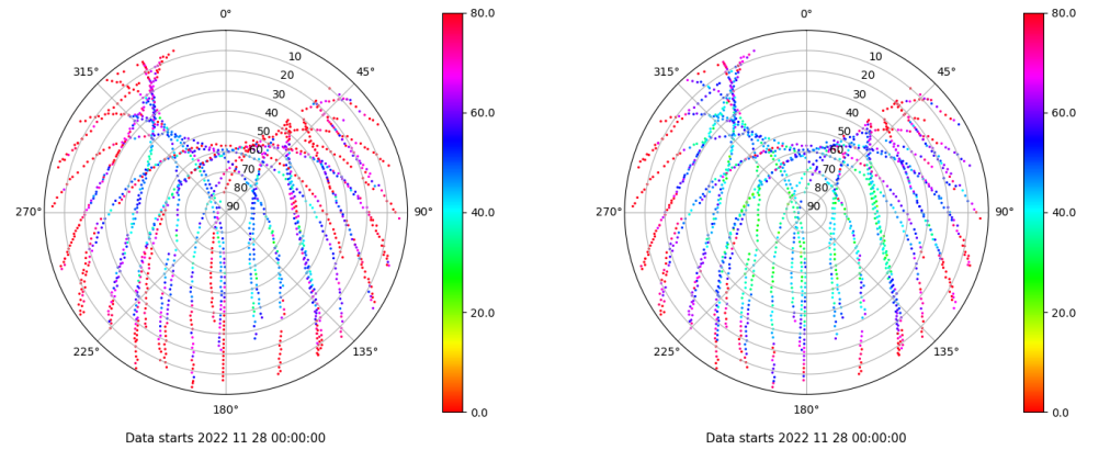
Skyplot for station ALC1. Parameter M1C Data file ALC100ESP_R_2022332.xtr Skyplot for station ALC1. Parameter M2C Data file ALC100ESP_R_2022332.xtr
