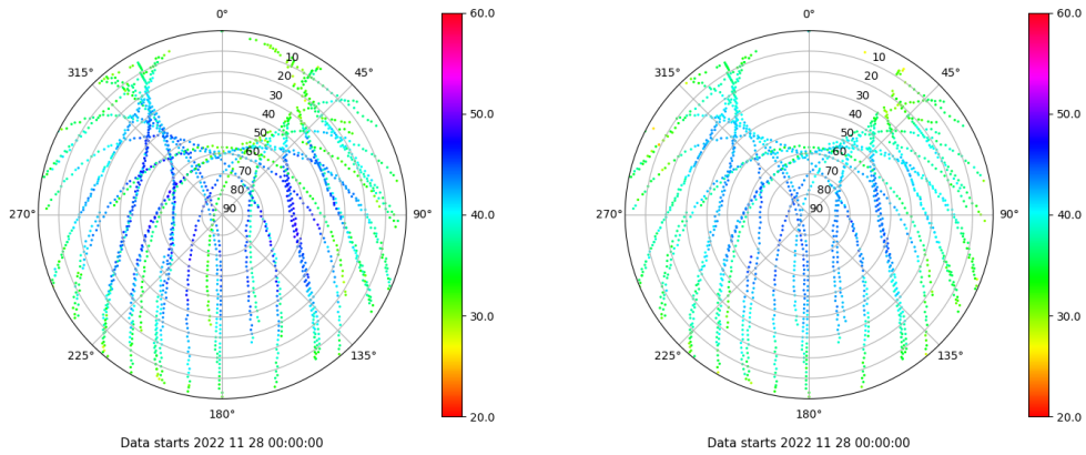
Skyplot for station ALC1. Signal to Noise S1C Data file ALC100ESP_R_2022332.xtr Skyplot for station ALC1. Signal to Noise S2C Data file ALC100ESP_R_2022332.xtr
