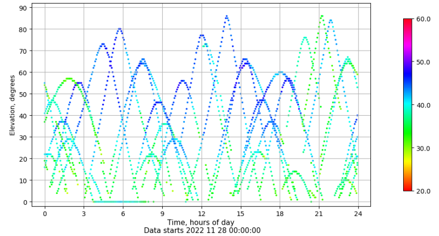
Time-elevation plot for station ALC1. Signal to Noise S1C Data file ALC100ESP_R_2022332.xtr
