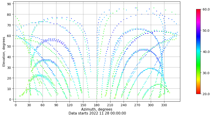
Azimuth-elevation plot for station ALC1. Signal to Noise S1C Data file ALC100ESP_R_2022332.xtr
