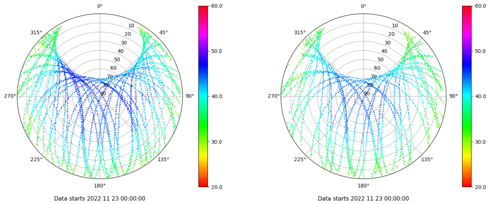
Skyplot for station ALC1. Signal to Noise S1C Data file ALC100ESP_R_2022327.xtr Skyplot for station ALC1. Signal to Noise S2X Data file ALC100ESP_R_2022327.xtr
