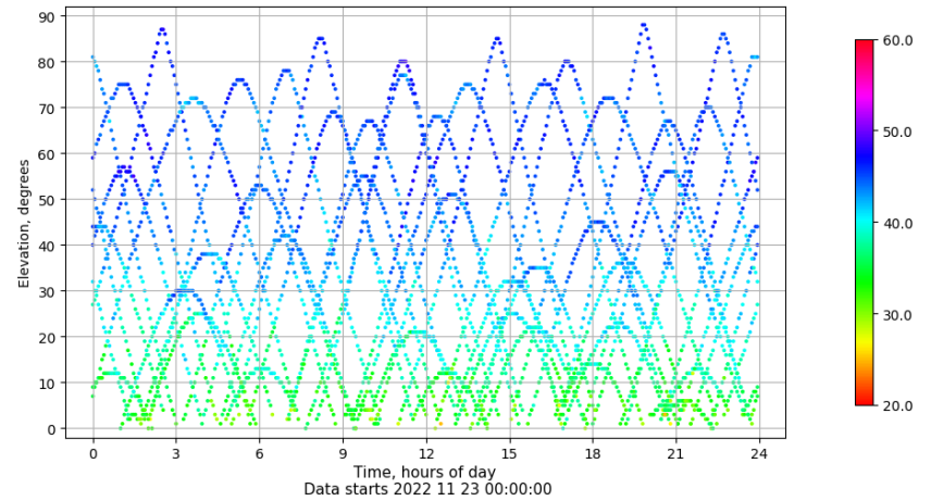
Time-elevation plot for station ALC1. Signal to Noise S1C Data file ALC100ESP_R_2022327.xtr
