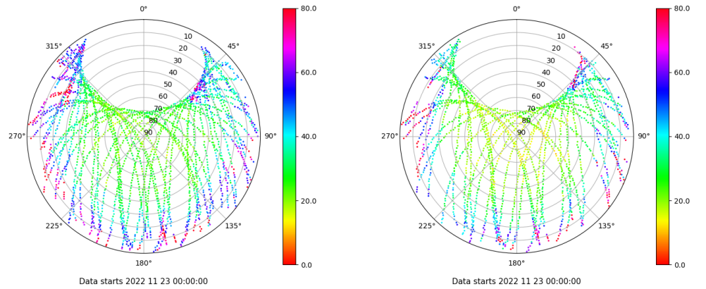
Skyplot for station ALC1. Parameter M1C Data file ALC100ESP_R_2022327.xtr Skyplot for station ALC1. Parameter M2X Data file ALC100ESP_R_2022327.xtr
