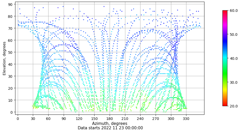
Azimuth-elevation plot for station ALC1. Signal to Noise S1C Data file ALC100ESP_R_2022327.xtr
