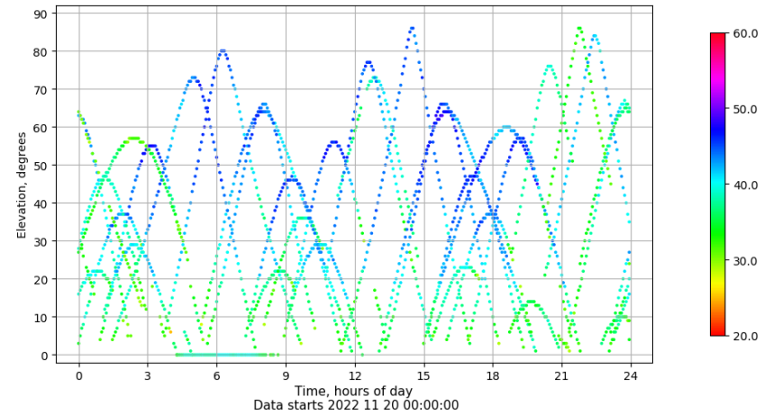
Time-elevation plot for station ALC1. Signal to Noise S1C Data file ALC100ESP_R_2022324.xtr
