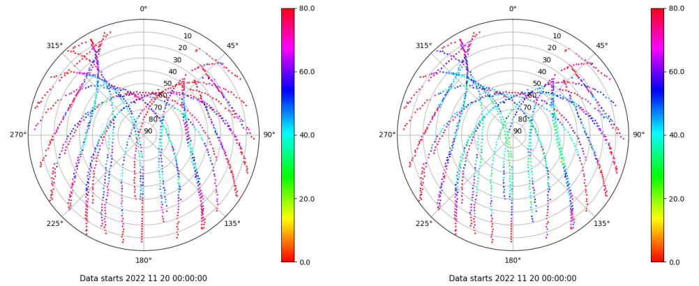
Skyplot for station ALC1. Parameter M1C Data file ALC100ESP_R_2022324.xtr Skyplot for station ALC1. Parameter M2C Data file ALC100ESP_R_2022324.xtr
