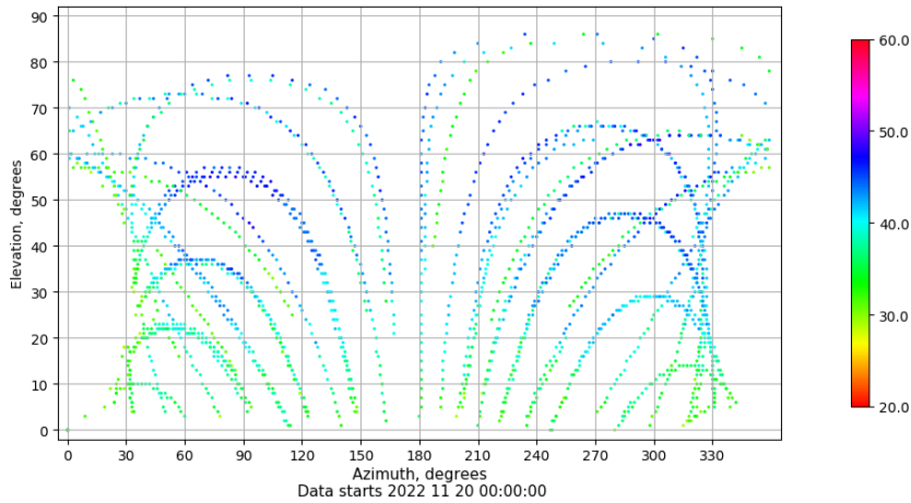
Azimuth-elevation plot for station ALC1. Signal to Noise S1C Data file ALC100ESP_R_2022324.xtr
