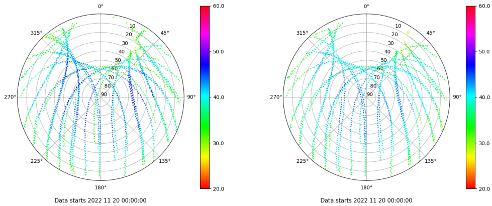
Skyplot for station ALC1. Signal to Noise S1C Data file ALC100ESP_R_2022324.xtr Skyplot for station ALC1. Signal to Noise S2C Data file ALC100ESP_R_2022324.xtr
