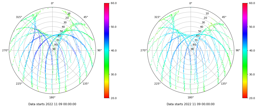
Skyplot for station ALC1. Signal to Noise S1C Data file ALC100ESP_R_2022313.xtr Skyplot for station ALC1. Signal to Noise S2C Data file ALC100ESP_R_2022313.xtr
