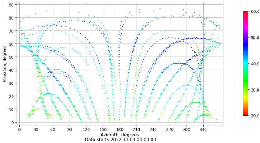
Azimuth-elevation plot for station ALC1. Signal to Noise S1C Data file ALC100ESP_R_2022313.xtr
