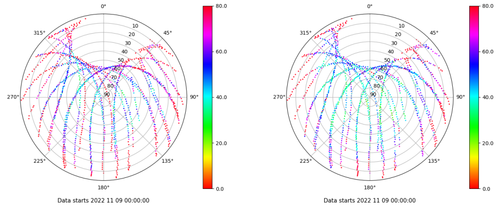
Skyplot for station ALC1. Parameter M1C Data file ALC100ESP_R_2022313.xtr Skyplot for station ALC1. Parameter M2C Data file ALC100ESP_R_2022313.xtr
