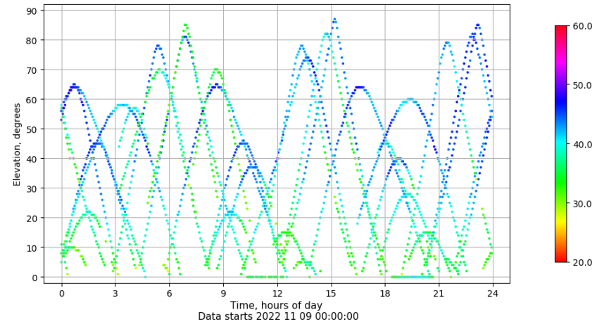
Time-elevation plot for station ALC1. Signal to Noise S1C Data file ALC100ESP_R_2022313.xtr
