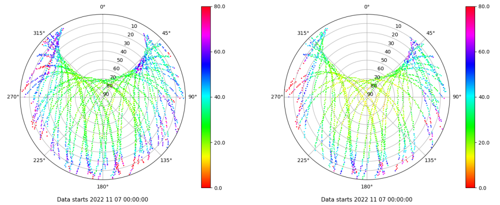
Skyplot for station ALC1. Parameter M1C Data file ALC100ESP_R_2022311.xtr Skyplot for station ALC1. Parameter M2X Data file ALC100ESP_R_2022311.xtr
