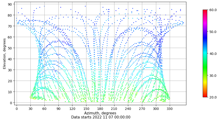
Azimuth-elevation plot for station ALC1. Signal to Noise S1C Data file ALC100ESP_R_2022311.xtr
