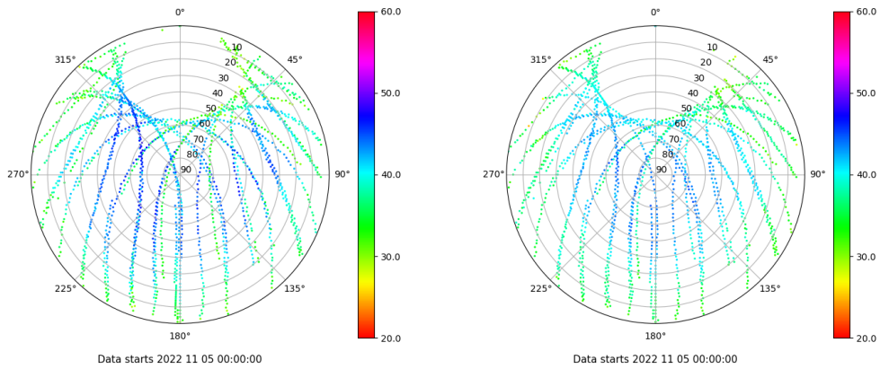
Skyplot for station ALC1. Signal to Noise S1C Data file ALC100ESP_R_2022309.xtr Skyplot for station ALC1. Signal to Noise S2C Data file ALC100ESP_R_2022309.xtr
