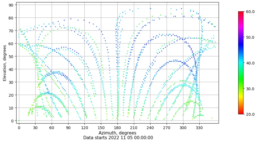
Azimuth-elevation plot for station ALC1. Signal to Noise S1C Data file ALC100ESP_R_2022309.xtr
