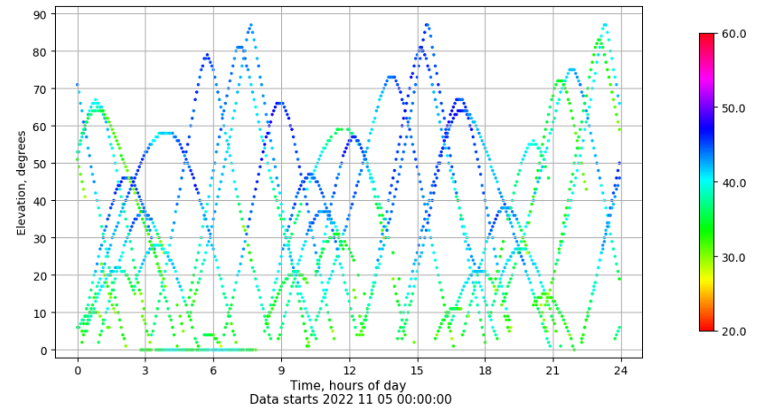
Time-elevation plot for station ALC1. Signal to Noise S1C Data file ALC100ESP_R_2022309.xtr
