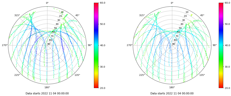
Skyplot for station ALC1. Signal to Noise S1C Data file ALC100ESP_R_2022308.xtr Skyplot for station ALC1. Signal to Noise S2C Data file ALC100ESP_R_2022308.xtr
