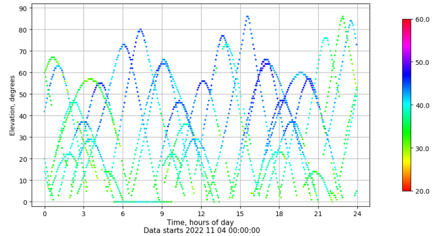
Time-elevation plot for station ALC1. Signal to Noise S1C Data file ALC100ESP_R_2022308.xtr
