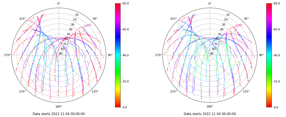
Skyplot for station ALC1. Parameter M1C Data file ALC100ESP_R_2022308.xtr Skyplot for station ALC1. Parameter M2C Data file ALC100ESP_R_2022308.xtr
