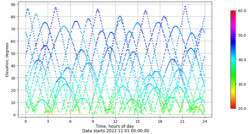
Time-elevation plot for station ALC1. Signal to Noise S1C Data file ALC100ESP_R_2022305.xtr
