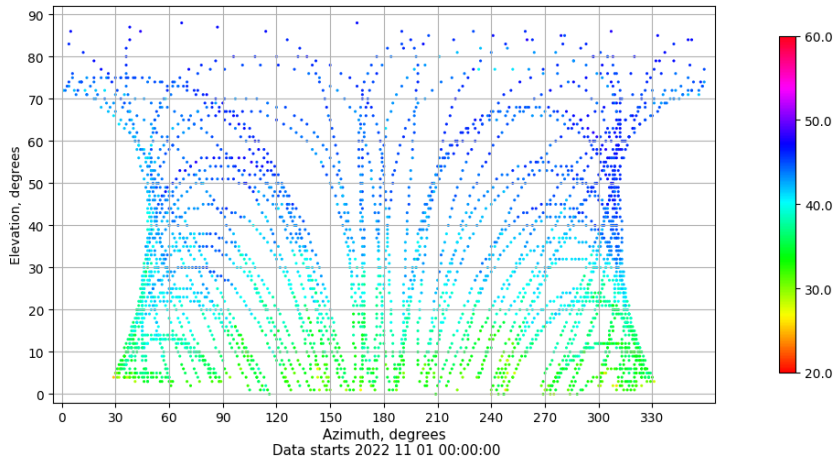
Azimuth-elevation plot for station ALC1. Signal to Noise S1C Data file ALC100ESP_R_2022305.xtr
