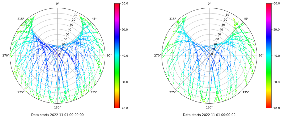
Skyplot for station ALC1. Signal to Noise S1C Data file ALC100ESP_R_2022305.xtr Skyplot for station ALC1. Signal to Noise S2X Data file ALC100ESP_R_2022305.xtr
