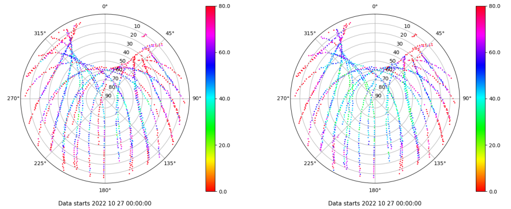
Skyplot for station ALC1. Parameter M1C Data file ALC100ESP_R_2022300.xtr Skyplot for station ALC1. Parameter M2C Data file ALC100ESP_R_2022300.xtr
