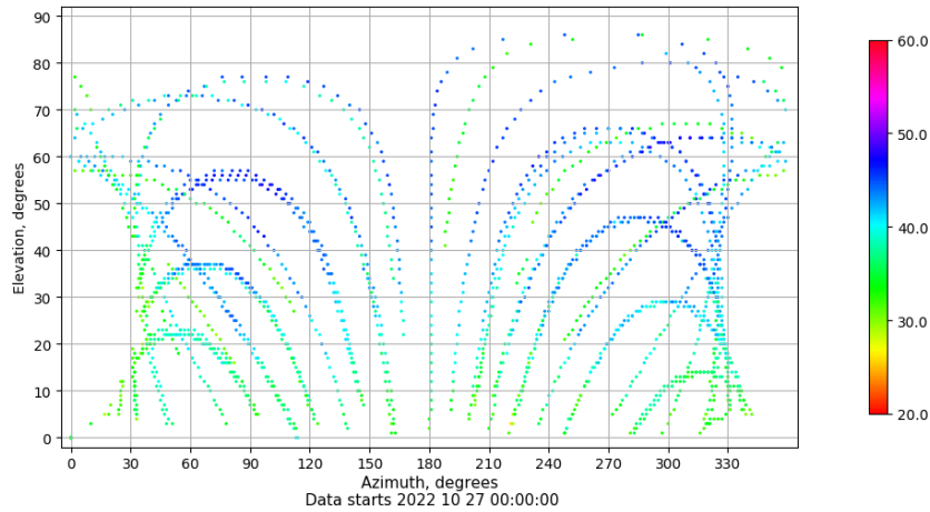
Azimuth-elevation plot for station ALC1. Signal to Noise S1C Data file ALC100ESP_R_2022300.xtr
