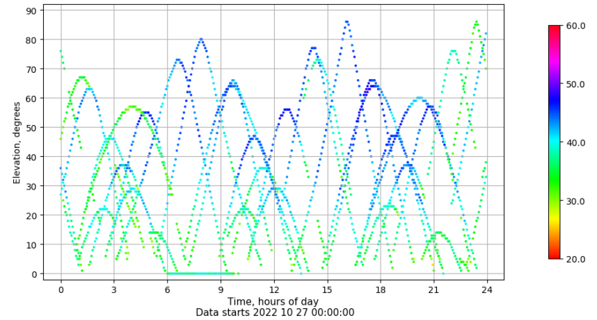
Time-elevation plot for station ALC1. Signal to Noise S1C Data file ALC100ESP_R_2022300.xtr
