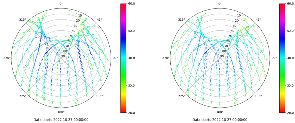
Skyplot for station ALC1. Signal to Noise S1C Data file ALC100ESP_R_2022300.xtr Skyplot for station ALC1. Signal to Noise S2C Data file ALC100ESP_R_2022300.xtr
