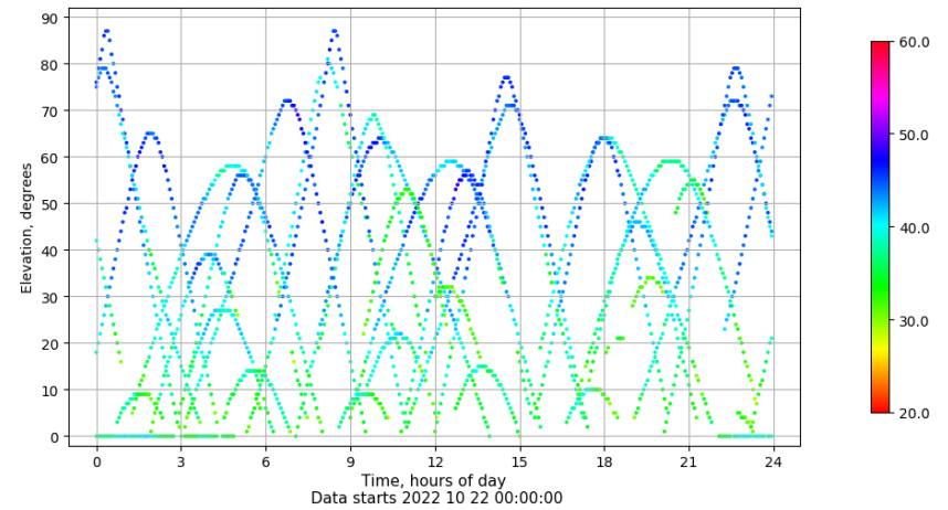
Time-elevation plot for station ALC1. Signal to Noise S1C Data file ALC100ESP_R_2022295.xtr
