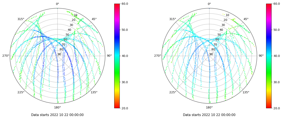
Skyplot for station ALC1. Signal to Noise S1C Data file ALC100ESP_R_2022295.xtr Skyplot for station ALC1. Signal to Noise S2C Data file ALC100ESP_R_2022295.xtr
