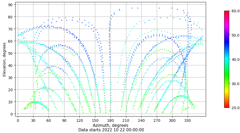
Azimuth-elevation plot for station ALC1. Signal to Noise S1C Data file ALC100ESP_R_2022295.xtr
