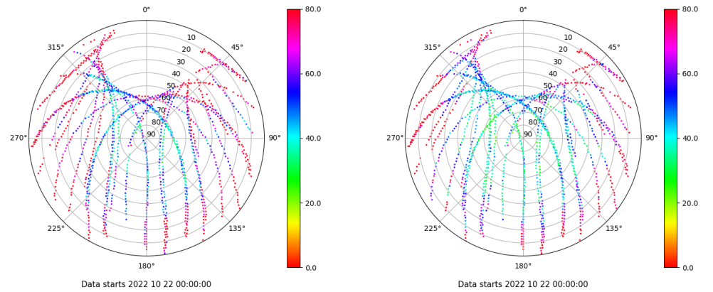
Skyplot for station ALC1. Parameter M1C Data file ALC100ESP_R_2022295.xtr Skyplot for station ALC1. Parameter M2C Data file ALC100ESP_R_2022295.xtr
