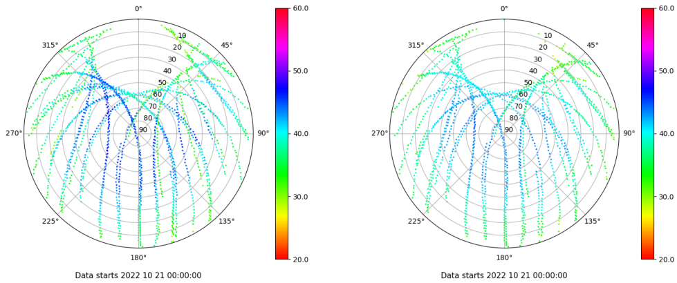
Skyplot for station ALC1. Signal to Noise S1C Data file ALC100ESP_R_2022294.xtr Skyplot for station ALC1. Signal to Noise S2C Data file ALC100ESP_R_2022294.xtr
