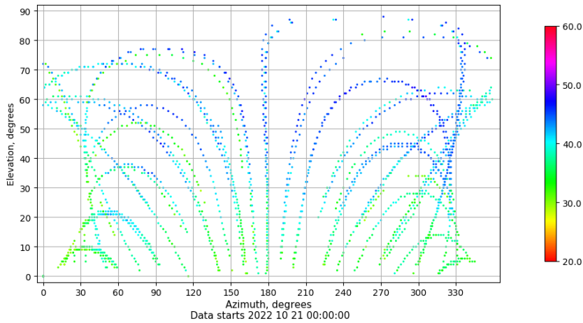
Azimuth-elevation plot for station ALC1. Signal to Noise S1C Data file ALC100ESP_R_2022294.xtr
