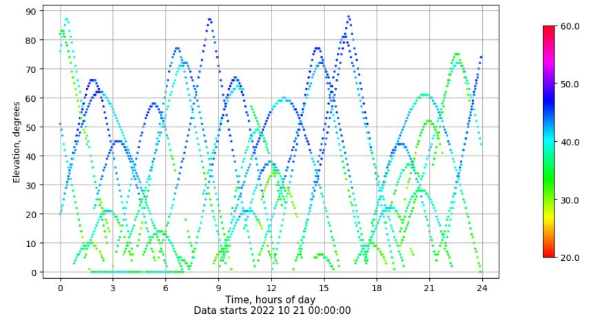
Time-elevation plot for station ALC1. Signal to Noise S1C Data file ALC100ESP_R_2022294.xtr
