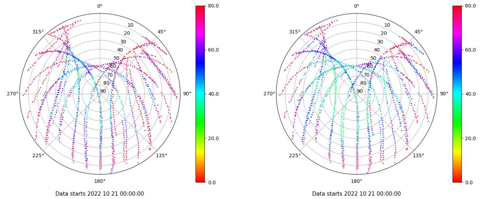
Skyplot for station ALC1. Parameter M1C Data file ALC100ESP_R_2022294.xtr Skyplot for station ALC1. Parameter M2C Data file ALC100ESP_R_2022294.xtr
