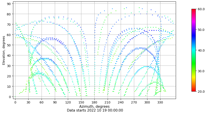
Azimuth-elevation plot for station ALC1. Signal to Noise S1C Data file ALC100ESP_R_2022292.xtr
