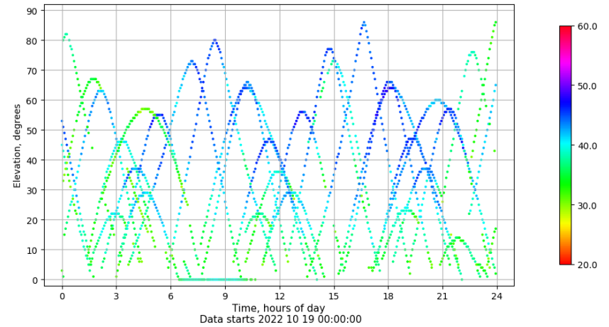
Time-elevation plot for station ALC1. Signal to Noise S1C Data file ALC100ESP_R_2022292.xtr
