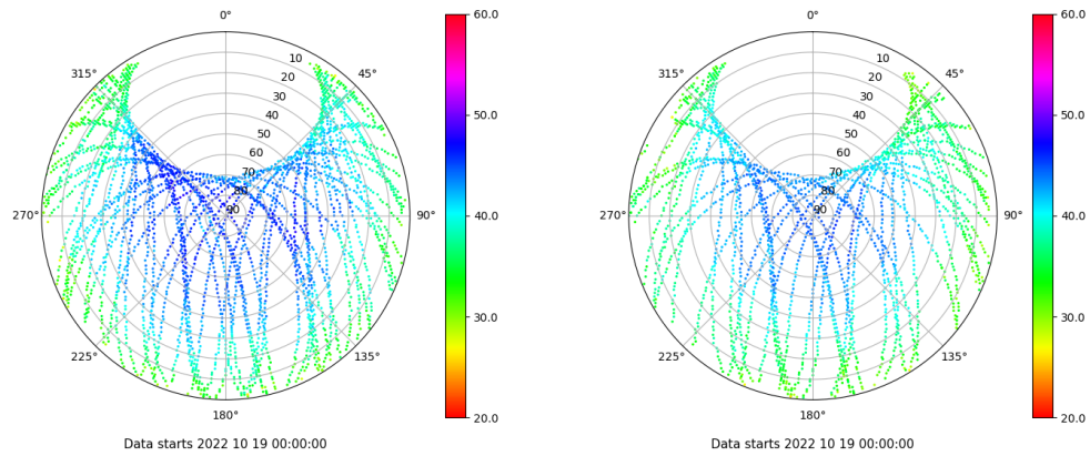
Skyplot for station ALC1. Signal to Noise S1C Data file ALC100ESP_R_2022292.xtr Skyplot for station ALC1. Signal to Noise S2X Data file ALC100ESP_R_2022292.xtr
