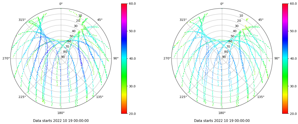
Skyplot for station ALC1. Signal to Noise S1C Data file ALC100ESP_R_2022292.xtr Skyplot for station ALC1. Signal to Noise S2C Data file ALC100ESP_R_2022292.xtr
