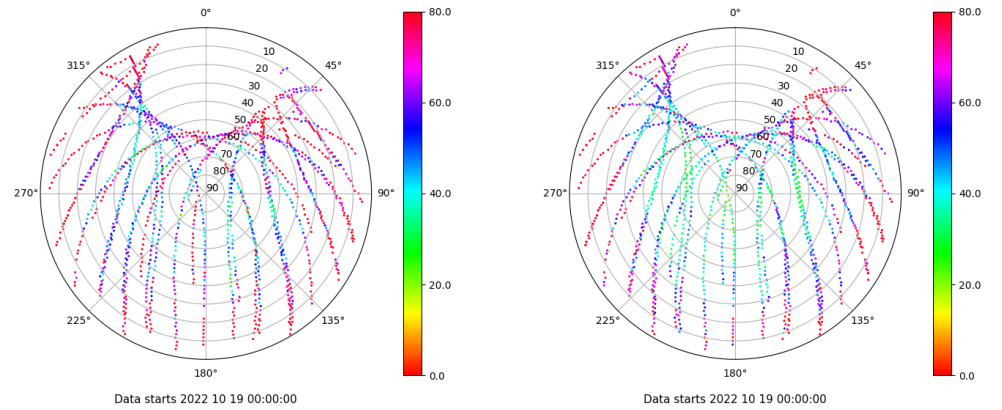
Skyplot for station ALC1. Parameter M1C Data file ALC100ESP_R_2022292.xtr Skyplot for station ALC1. Parameter M2C Data file ALC100ESP_R_2022292.xtr
