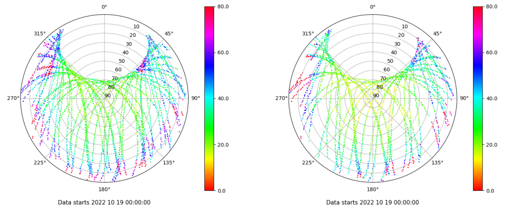
Skyplot for station ALC1. Parameter M1C Data file ALC100ESP_R_2022292.xtr Skyplot for station ALC1. Parameter M2X Data file ALC100ESP_R_2022292.xtr
