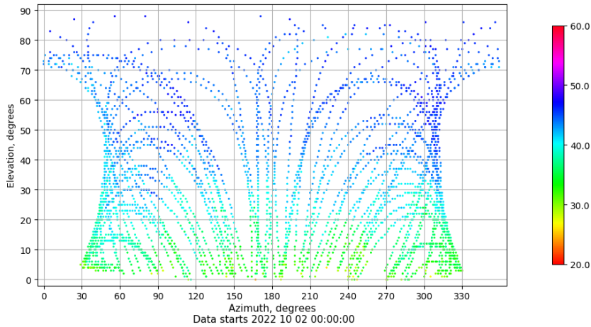
Azimuth-elevation plot for station ALC1. Signal to Noise S1C Data file ALC100ESP_R_2022275.xtr
