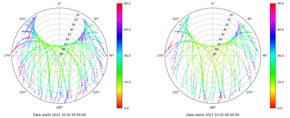
Skyplot for station ALC1. Parameter M1C Data file ALC100ESP_R_2022275.xtr Skyplot for station ALC1. Parameter M2X Data file ALC100ESP_R_2022275.xtr
