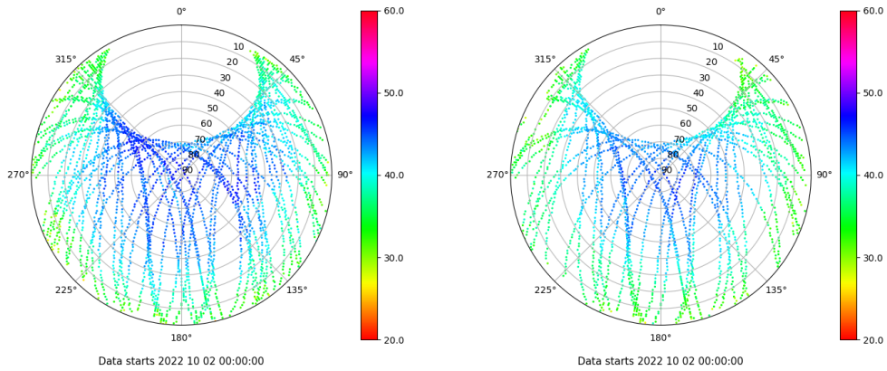
Skyplot for station ALC1. Signal to Noise S1C Data file ALC100ESP_R_2022275.xtr Skyplot for station ALC1. Signal to Noise S2X Data file ALC100ESP_R_2022275.xtr
