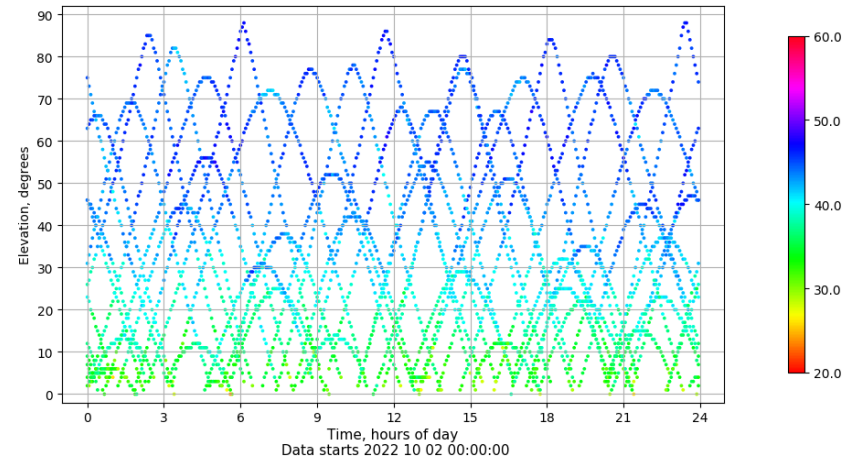
Time-elevation plot for station ALC1. Signal to Noise S1C Data file ALC100ESP_R_2022275.xtr
