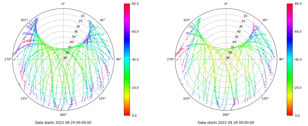
Skyplot for station ALC1. Parameter M1C Data file ALC100ESP_R_2022272.xtr Skyplot for station ALC1. Parameter M2X Data file ALC100ESP_R_2022272.xtr
