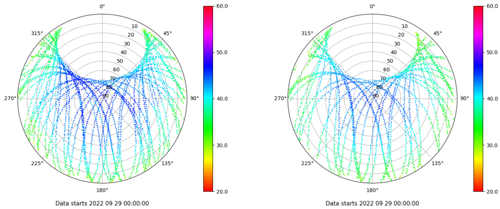
Skyplot for station ALC1. Signal to Noise S1C Data file ALC100ESP_R_2022272.xtr Skyplot for station ALC1. Signal to Noise S2X Data file ALC100ESP_R_2022272.xtr
