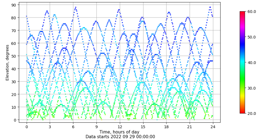
Time-elevation plot for station ALC1. Signal to Noise S1C Data file ALC100ESP_R_2022272.xtr
