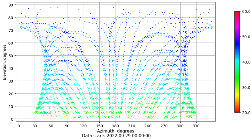
Azimuth-elevation plot for station ALC1. Signal to Noise S1C Data file ALC100ESP_R_2022272.xtr
