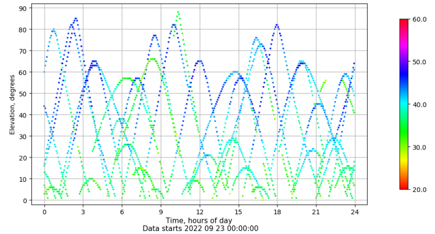
Time-elevation plot for station ALC1. Signal to Noise S1C Data file ALC100ESP_R_2022266.xtr
