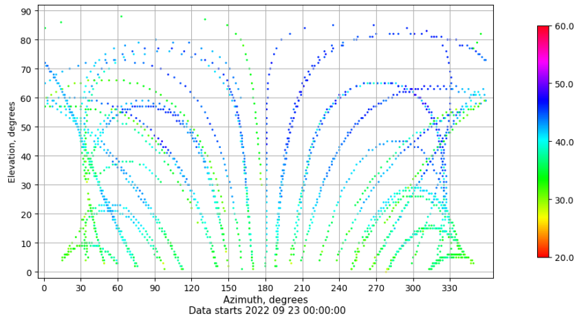
Azimuth-elevation plot for station ALC1. Signal to Noise S1C Data file ALC100ESP_R_2022266.xtr
