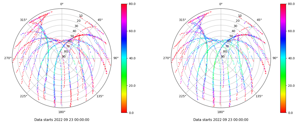
Skyplot for station ALC1. Parameter M1C Data file ALC100ESP_R_2022266.xtr Skyplot for station ALC1. Parameter M2C Data file ALC100ESP_R_2022266.xtr
