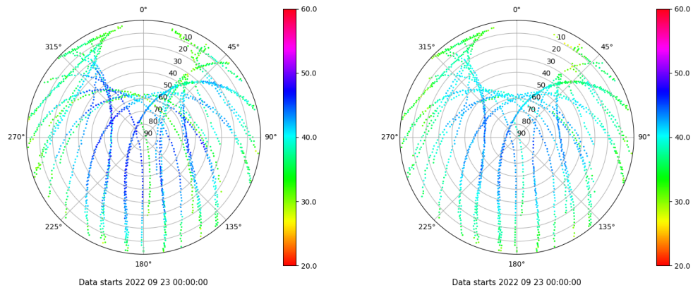
Skyplot for station ALC1. Signal to Noise S1C Data file ALC100ESP_R_2022266.xtr Skyplot for station ALC1. Signal to Noise S2C Data file ALC100ESP_R_2022266.xtr
