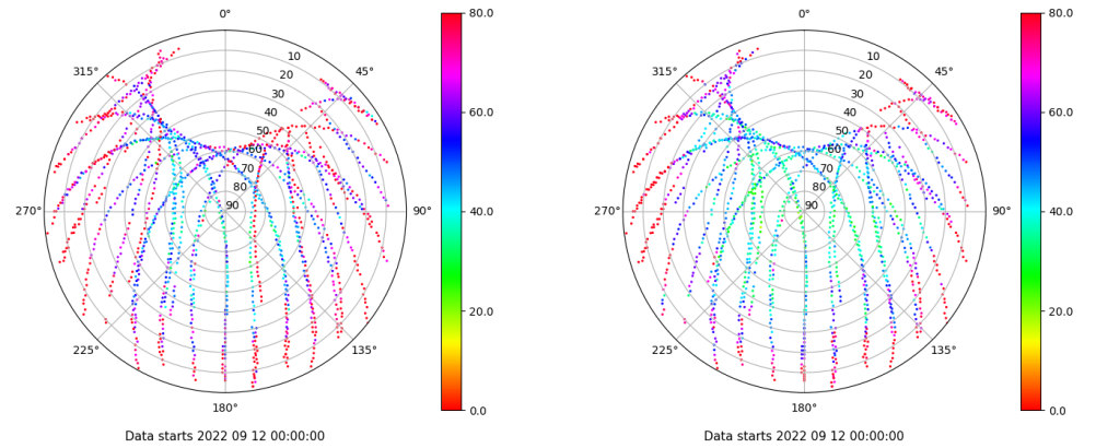
Skyplot for station ALC1. Parameter M1C Data file ALC100ESP_R_2022255.xtr Skyplot for station ALC1. Parameter M2C Data file ALC100ESP_R_2022255.xtr
