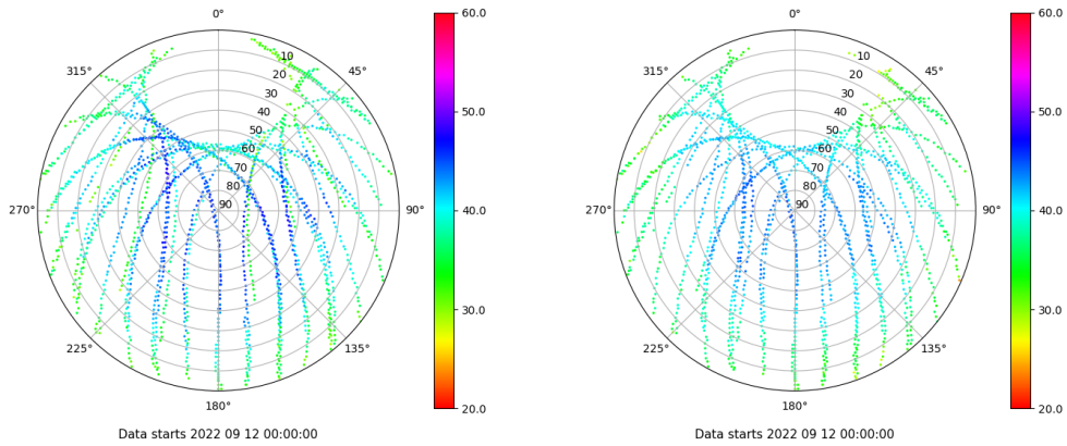
Skyplot for station ALC1. Signal to Noise S1C Data file ALC100ESP_R_2022255.xtr Skyplot for station ALC1. Signal to Noise S2C Data file ALC100ESP_R_2022255.xtr
