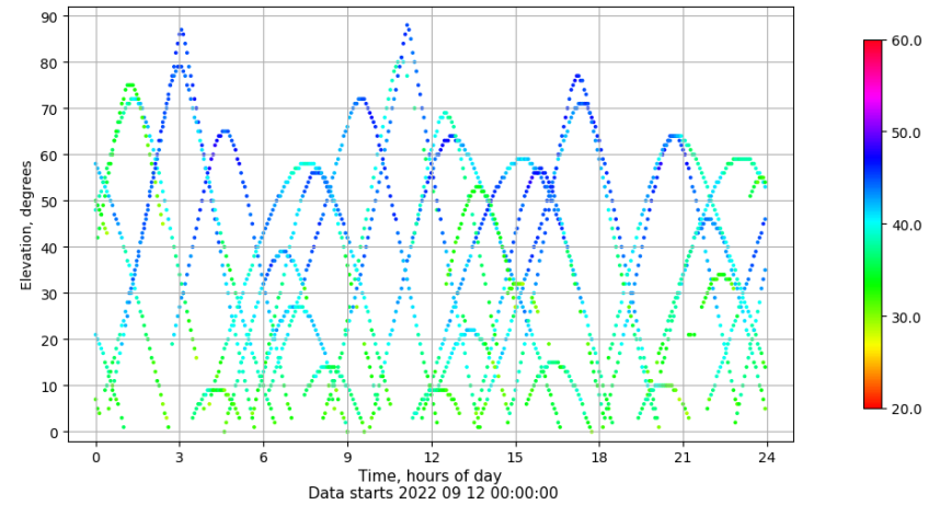
Time-elevation plot for station ALC1. Signal to Noise S1C Data file ALC100ESP_R_2022255.xtr
