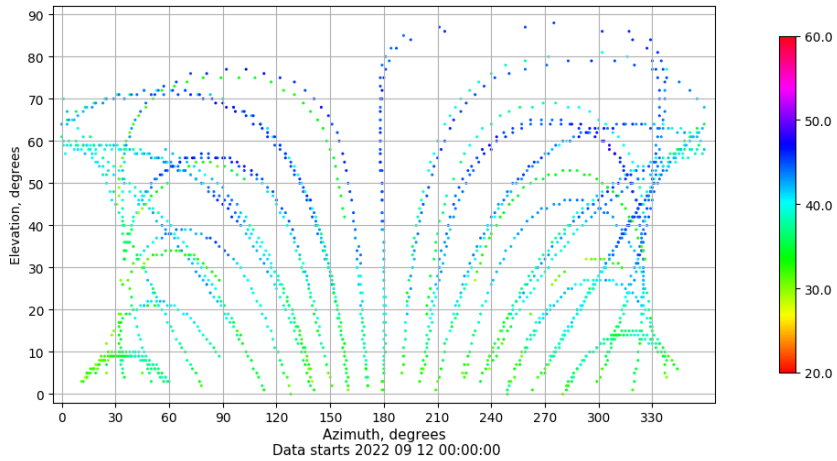
Azimuth-elevation plot for station ALC1. Signal to Noise S1C Data file ALC100ESP_R_2022255.xtr
