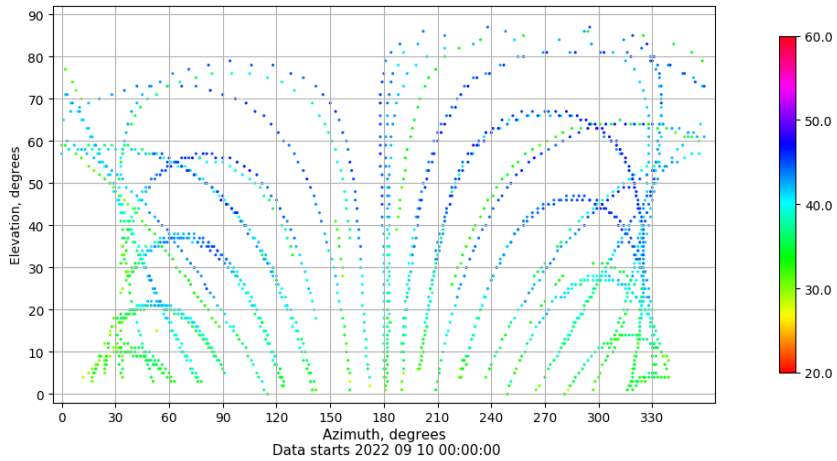
Azimuth-elevation plot for station ALC1. Signal to Noise S1C Data file ALC100ESP_R_2022253.xtr
