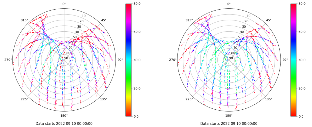
Skyplot for station ALC1. Parameter M1C Data file ALC100ESP_R_2022253.xtr Skyplot for station ALC1. Parameter M2C Data file ALC100ESP_R_2022253.xtr
