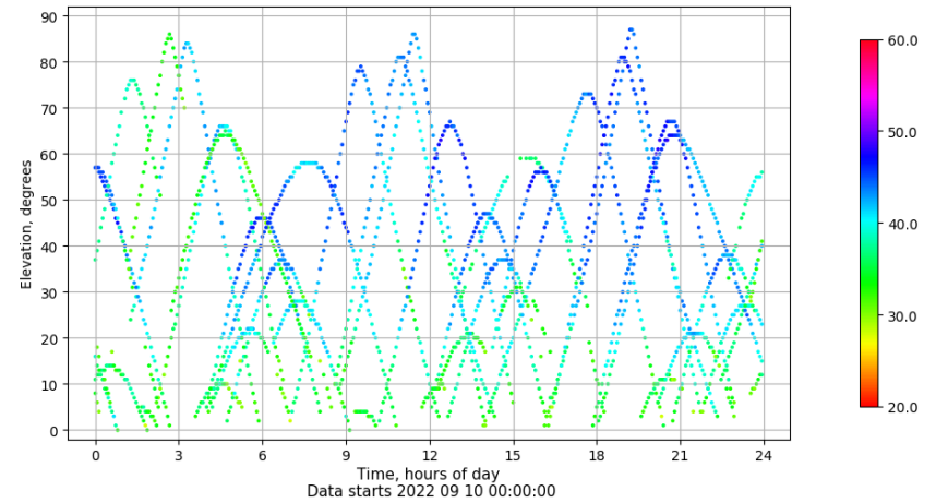
Time-elevation plot for station ALC1. Signal to Noise S1C Data file ALC100ESP_R_2022253.xtr
