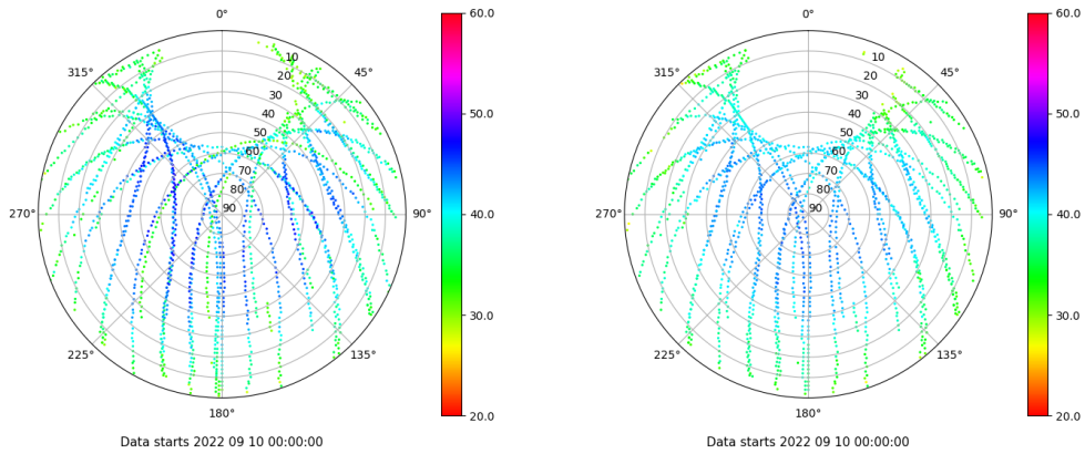
Skyplot for station ALC1. Signal to Noise S1C Data file ALC100ESP_R_2022253.xtr Skyplot for station ALC1. Signal to Noise S2C Data file ALC100ESP_R_2022253.xtr
