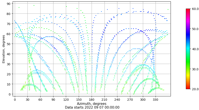
Azimuth-elevation plot for station ALC1. Signal to Noise S1C Data file ALC100ESP_R_2022250.xtr
