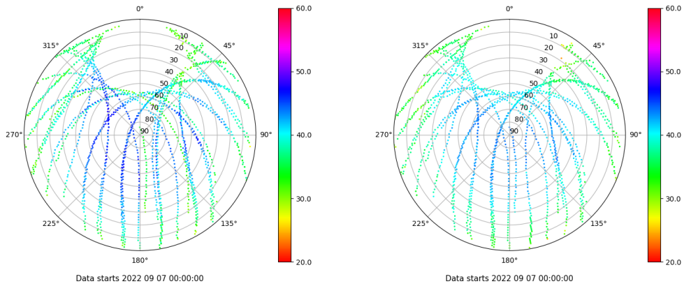
Skyplot for station ALC1. Signal to Noise S1C Data file ALC100ESP_R_2022250.xtr Skyplot for station ALC1. Signal to Noise S2C Data file ALC100ESP_R_2022250.xtr
