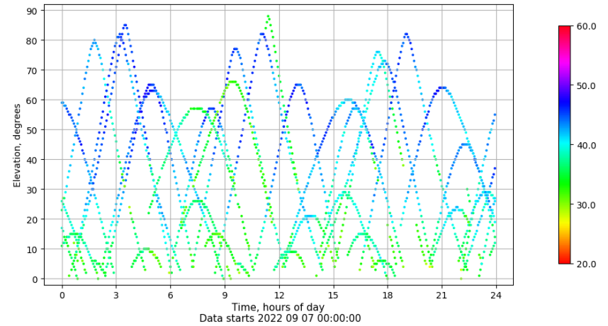
Time-elevation plot for station ALC1. Signal to Noise S1C Data file ALC100ESP_R_2022250.xtr
