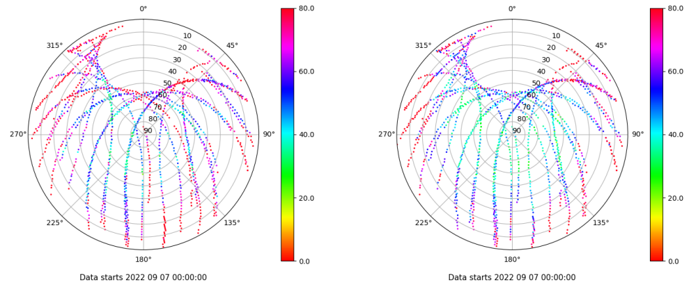
Skyplot for station ALC1. Parameter M1C Data file ALC100ESP_R_2022250.xtr Skyplot for station ALC1. Parameter M2C Data file ALC100ESP_R_2022250.xtr
