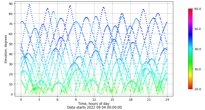
Time-elevation plot for station ALC1. Signal to Noise S1C Data file ALC100ESP_R_2022247.xtr
