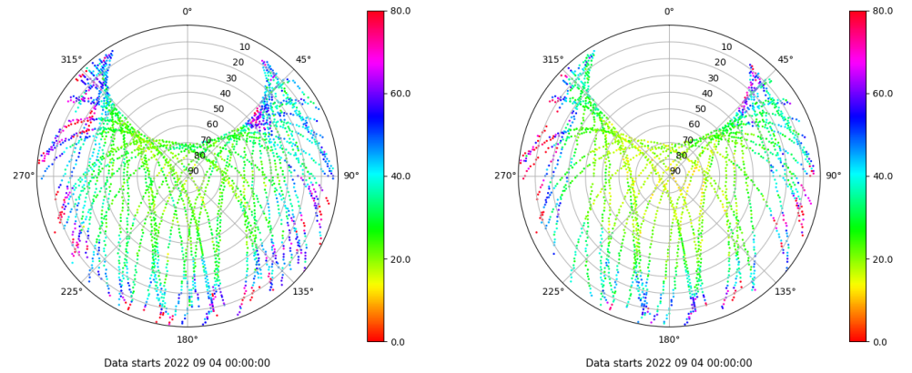
Skyplot for station ALC1. Parameter M1C Data file ALC100ESP_R_2022247.xtr Skyplot for station ALC1. Parameter M2X Data file ALC100ESP_R_2022247.xtr
