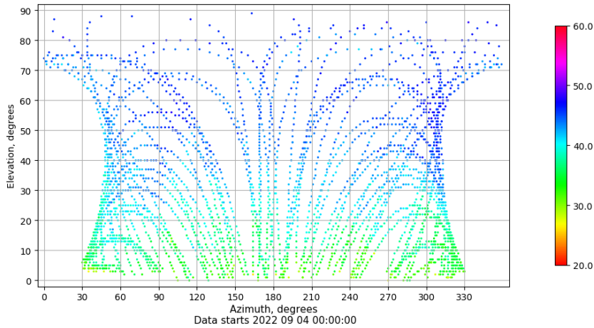
Azimuth-elevation plot for station ALC1. Signal to Noise S1C Data file ALC100ESP_R_2022247.xtr
