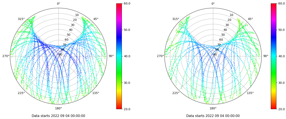
Skyplot for station ALC1. Signal to Noise S1C Data file ALC100ESP_R_2022247.xtr Skyplot for station ALC1. Signal to Noise S2X Data file ALC100ESP_R_2022247.xtr
