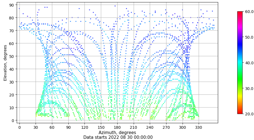
Azimuth-elevation plot for station ALC1. Signal to Noise S1C Data file ALC100ESP_R_2022242.xtr
