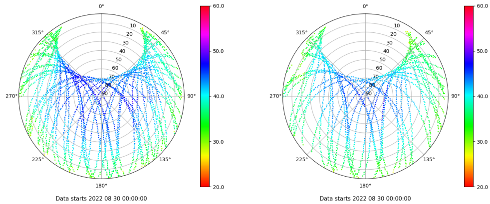
Skyplot for station ALC1. Signal to Noise S1C Data file ALC100ESP_R_2022242.xtr Skyplot for station ALC1. Signal to Noise S2X Data file ALC100ESP_R_2022242.xtr
