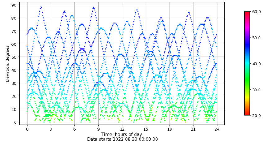
Time-elevation plot for station ALC1. Signal to Noise S1C Data file ALC100ESP_R_2022242.xtr
