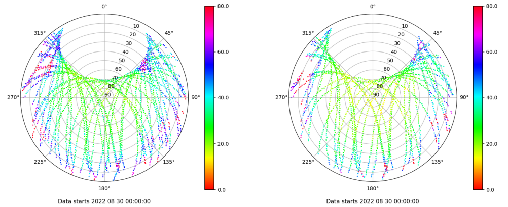
Skyplot for station ALC1. Parameter M1C Data file ALC100ESP_R_2022242.xtr Skyplot for station ALC1. Parameter M2X Data file ALC100ESP_R_2022242.xtr
