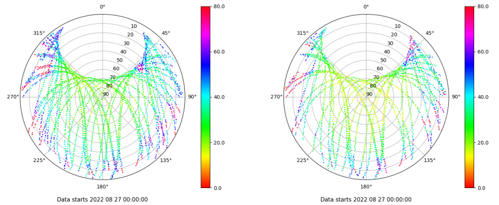
Skyplot for station ALC1. Parameter M1C Data file ALC100ESP_R_2022239.xtr Skyplot for station ALC1. Parameter M2X Data file ALC100ESP_R_2022239.xtr
