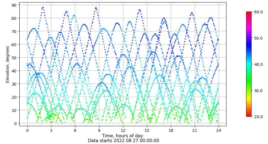
Time-elevation plot for station ALC1. Signal to Noise S1C Data file ALC100ESP_R_2022239.xtr
