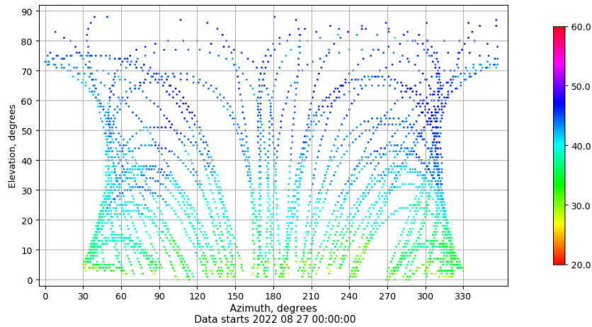
Azimuth-elevation plot for station ALC1. Signal to Noise S1C Data file ALC100ESP_R_2022239.xtr
