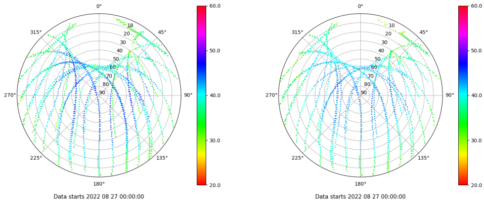
Skyplot for station ALC1. Signal to Noise S1C Data file ALC100ESP_R_2022239.xtr Skyplot for station ALC1. Signal to Noise S2C Data file ALC100ESP_R_2022239.xtr
