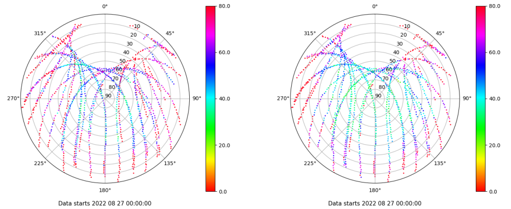
Skyplot for station ALC1. Parameter M1C Data file ALC100ESP_R_2022239.xtr Skyplot for station ALC1. Parameter M2C Data file ALC100ESP_R_2022239.xtr
