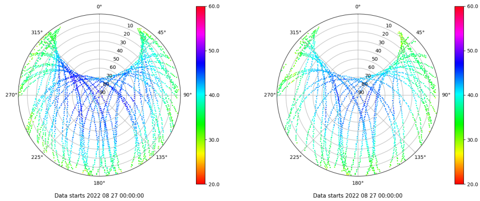
Skyplot for station ALC1. Signal to Noise S1C Data file ALC100ESP_R_2022239.xtr Skyplot for station ALC1. Signal to Noise S2X Data file ALC100ESP_R_2022239.xtr
