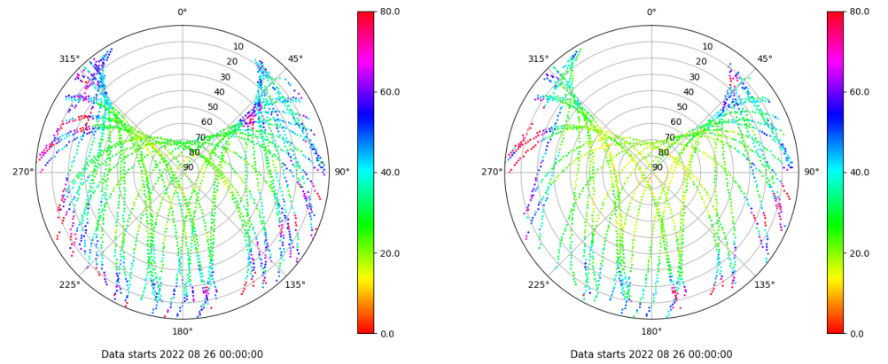
Skyplot for station ALC1. Parameter M1C Data file ALC100ESP_R_2022238.xtr Skyplot for station ALC1. Parameter M2X Data file ALC100ESP_R_2022238.xtr
