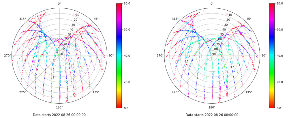
Skyplot for station ALC1. Parameter M1C Data file ALC100ESP_R_2022238.xtr Skyplot for station ALC1. Parameter M2C Data file ALC100ESP_R_2022238.xtr
