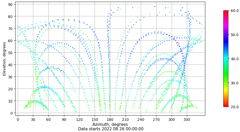
Azimuth-elevation plot for station ALC1. Signal to Noise S1C Data file ALC100ESP_R_2022238.xtr
