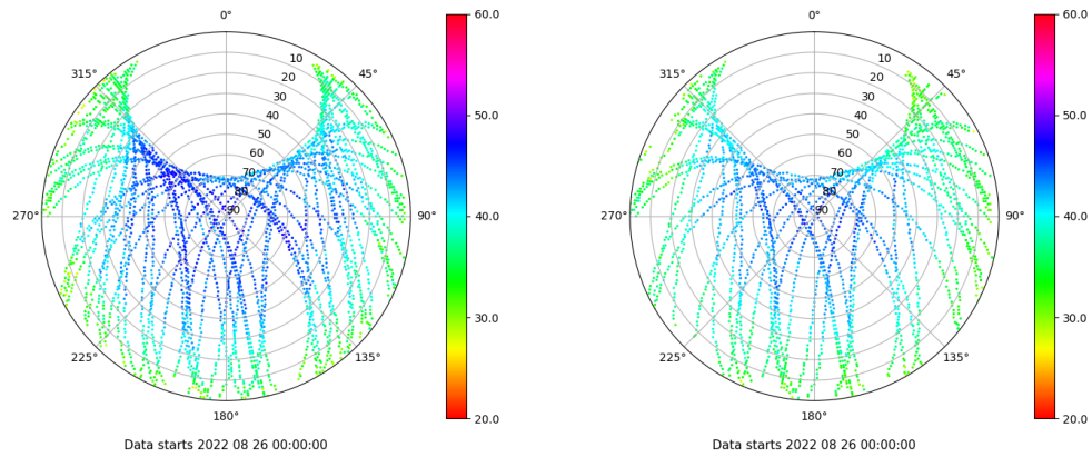
Skyplot for station ALC1. Signal to Noise S1C Data file ALC100ESP_R_2022238.xtr Skyplot for station ALC1. Signal to Noise S2X Data file ALC100ESP_R_2022238.xtr
