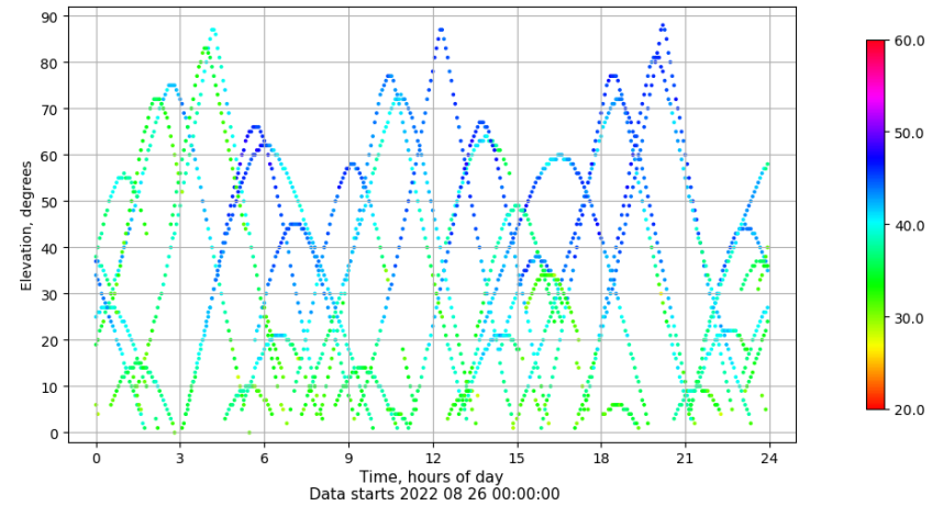
Time-elevation plot for station ALC1. Signal to Noise S1C Data file ALC100ESP_R_2022238.xtr
