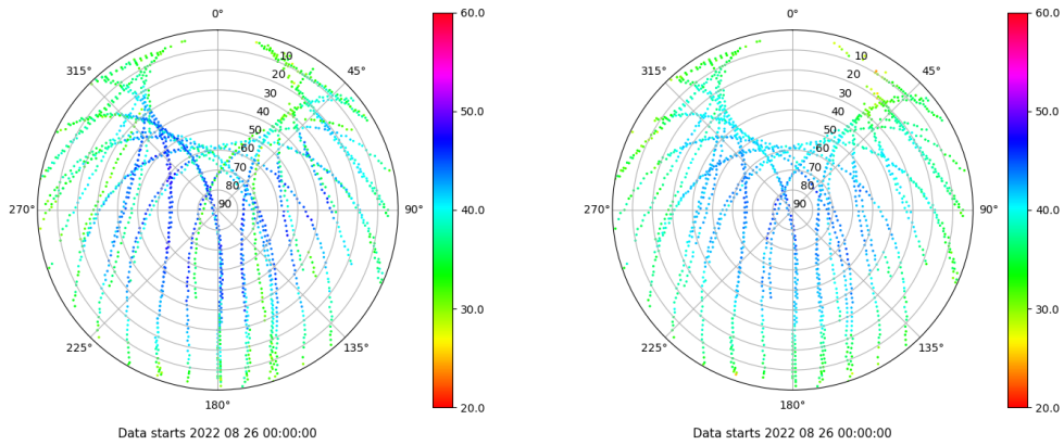
Skyplot for station ALC1. Signal to Noise S1C Data file ALC100ESP_R_2022238.xtr Skyplot for station ALC1. Signal to Noise S2C Data file ALC100ESP_R_2022238.xtr
