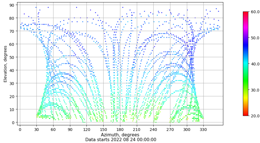
Azimuth-elevation plot for station ALC1. Signal to Noise S1C Data file ALC100ESP_R_2022236.xtr
