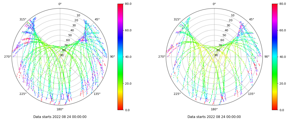
Skyplot for station ALC1. Parameter M1C Data file ALC100ESP_R_2022236.xtr Skyplot for station ALC1. Parameter M2X Data file ALC100ESP_R_2022236.xtr
