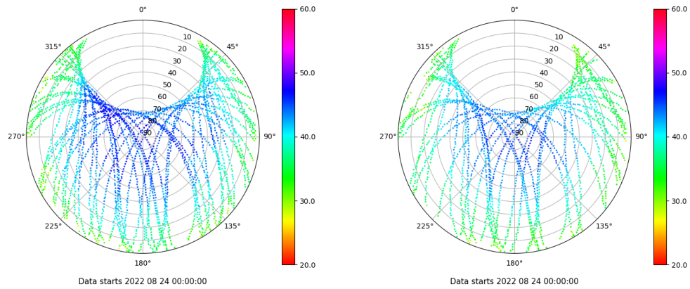
Skyplot for station ALC1. Signal to Noise S1C Data file ALC100ESP_R_2022236.xtr Skyplot for station ALC1. Signal to Noise S2X Data file ALC100ESP_R_2022236.xtr
