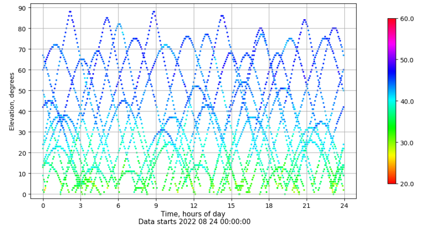
Time-elevation plot for station ALC1. Signal to Noise S1C Data file ALC100ESP_R_2022236.xtr
