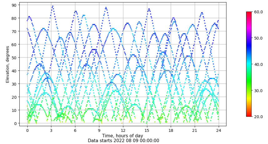
Time-elevation plot for station ALC1. Signal to Noise S1C Data file ALC100ESP_R_2022221.xtr
