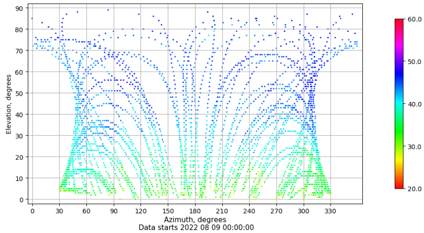
Azimuth-elevation plot for station ALC1. Signal to Noise S1C Data file ALC100ESP_R_2022221.xtr
