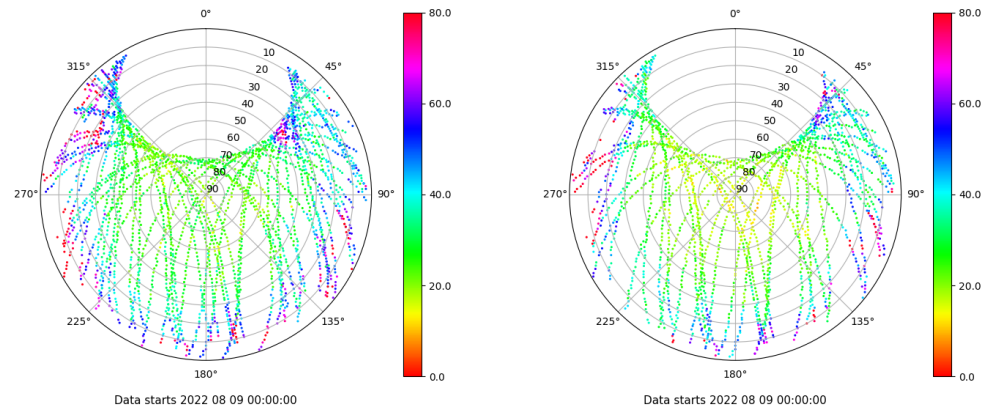
Skyplot for station ALC1. Parameter M1C Data file ALC100ESP_R_2022221.xtr Skyplot for station ALC1. Parameter M2X Data file ALC100ESP_R_2022221.xtr
