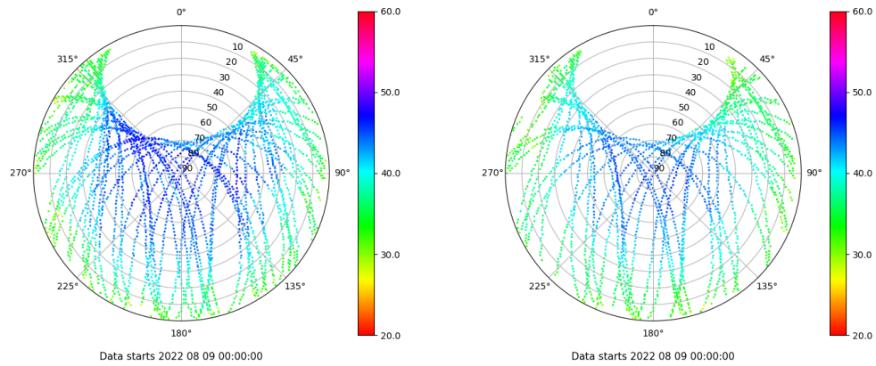
Skyplot for station ALC1. Signal to Noise S1C Data file ALC100ESP_R_2022221.xtr Skyplot for station ALC1. Signal to Noise S2X Data file ALC100ESP_R_2022221.xtr
