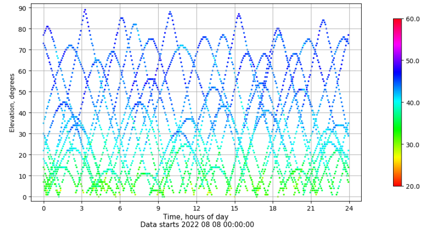
Time-elevation plot for station ALC1. Signal to Noise S1C Data file ALC100ESP_R_2022220.xtr
