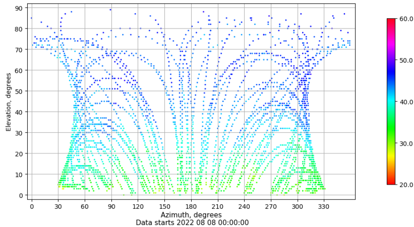
Azimuth-elevation plot for station ALC1. Signal to Noise S1C Data file ALC100ESP_R_2022220.xtr
