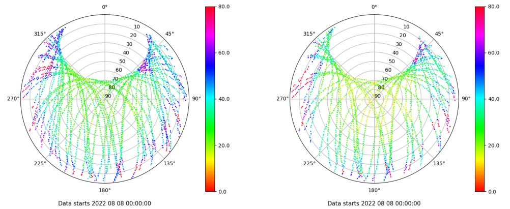
Skyplot for station ALC1. Parameter M1C Data file ALC100ESP_R_2022220.xtr Skyplot for station ALC1. Parameter M2X Data file ALC100ESP_R_2022220.xtr
