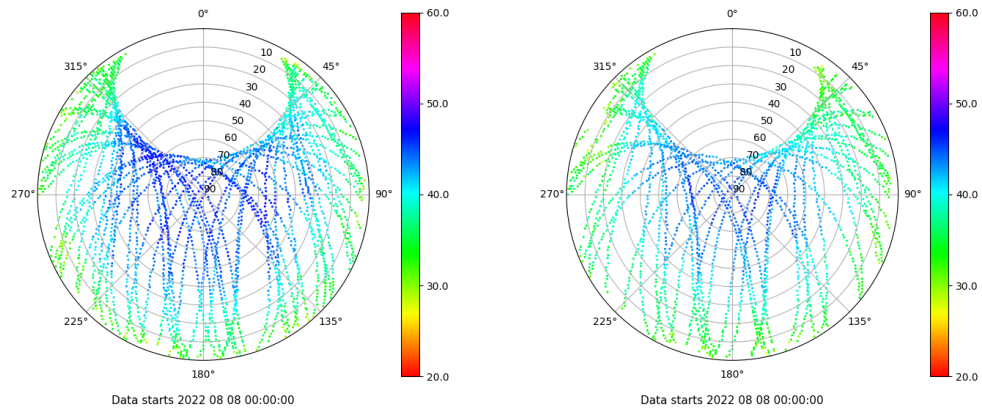
Skyplot for station ALC1. Signal to Noise S1C Data file ALC100ESP_R_2022220.xtr Skyplot for station ALC1. Signal to Noise S2X Data file ALC100ESP_R_2022220.xtr
