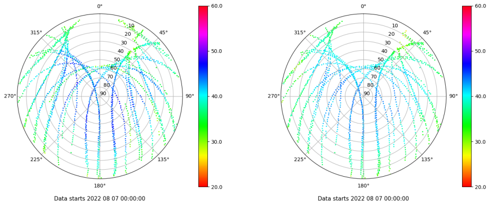
Skyplot for station ALC1. Signal to Noise S1C Data file ALC100ESP_R_2022219.xtr Skyplot for station ALC1. Signal to Noise S2C Data file ALC100ESP_R_2022219.xtr
