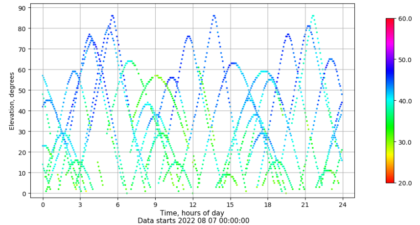
Time-elevation plot for station ALC1. Signal to Noise S1C Data file ALC100ESP_R_2022219.xtr
