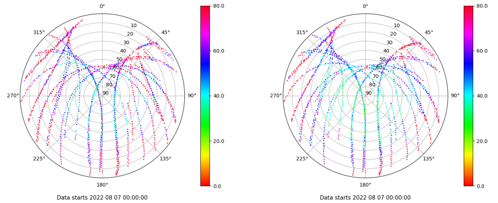
Skyplot for station ALC1. Parameter M1C Data file ALC100ESP_R_2022219.xtr Skyplot for station ALC1. Parameter M2C Data file ALC100ESP_R_2022219.xtr
