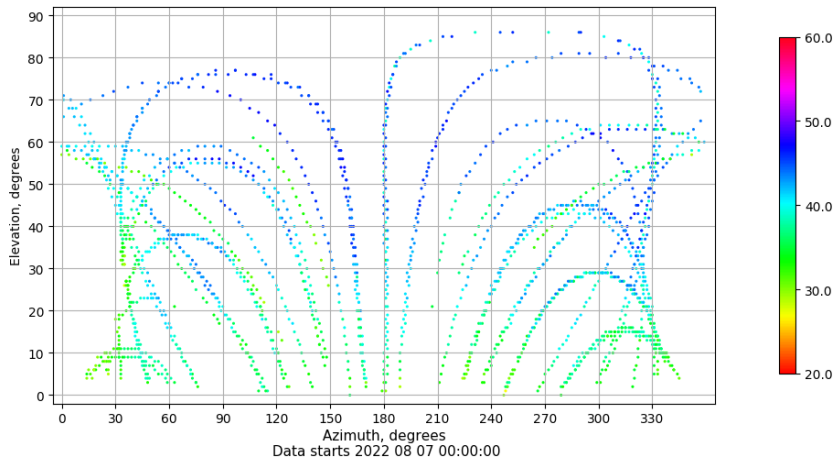
Azimuth-elevation plot for station ALC1. Signal to Noise S1C Data file ALC100ESP_R_2022219.xtr
