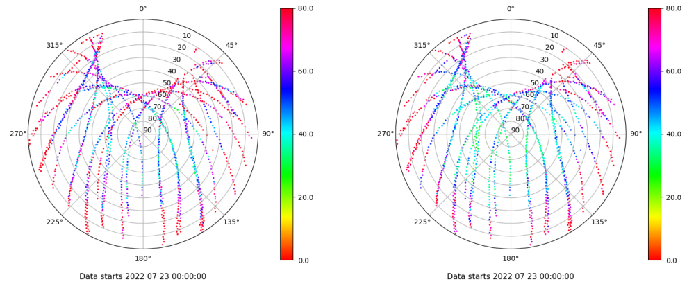
Skyplot for station ALC1. Parameter M1C Data file ALC100ESP_R_2022204.xtr Skyplot for station ALC1. Parameter M2C Data file ALC100ESP_R_2022204.xtr
