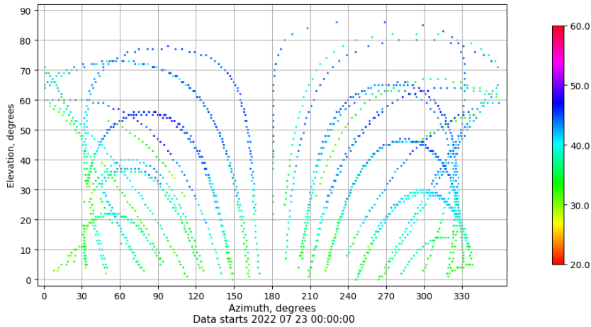
Azimuth-elevation plot for station ALC1. Signal to Noise S1C Data file ALC100ESP_R_2022204.xtr
