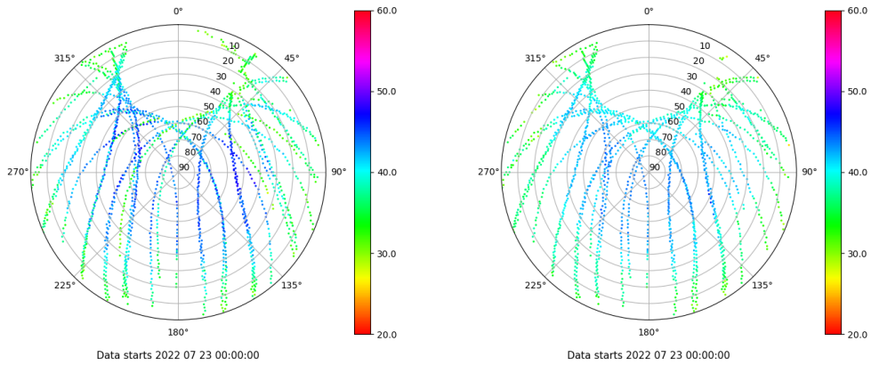
Skyplot for station ALC1. Signal to Noise S1C Data file ALC100ESP_R_2022204.xtr Skyplot for station ALC1. Signal to Noise S2C Data file ALC100ESP_R_2022204.xtr
