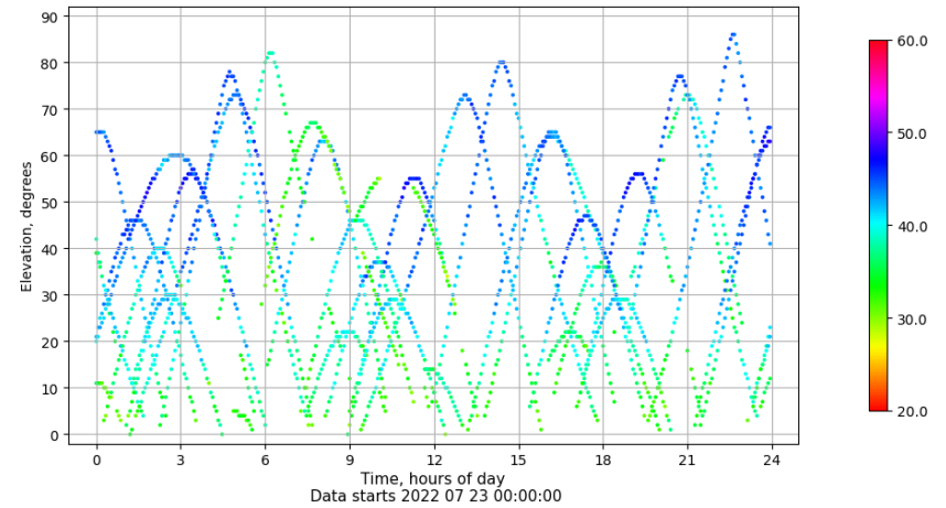
Time-elevation plot for station ALC1. Signal to Noise S1C Data file ALC100ESP_R_2022204.xtr
