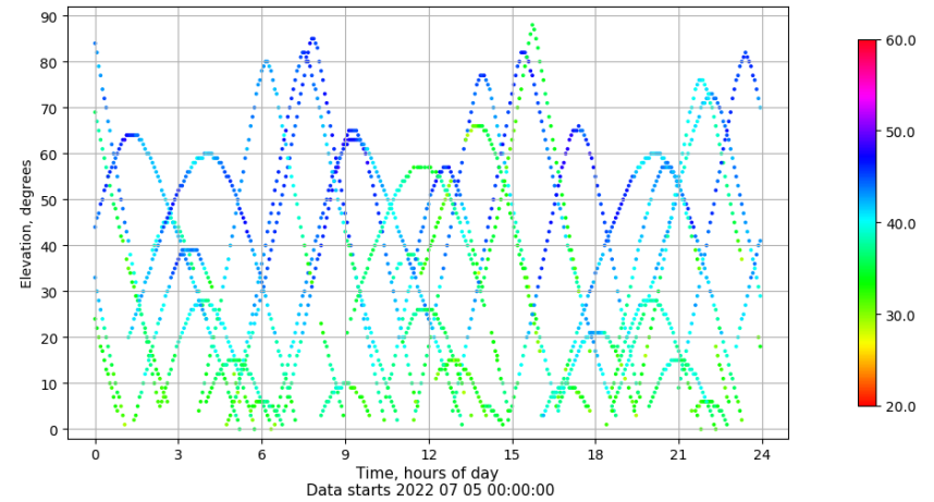
Time-elevation plot for station ALC1. Signal to Noise S1C Data file ALC100ESP_R_2022186.xtr
