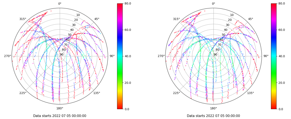
Skyplot for station ALC1. Parameter M1C Data file ALC100ESP_R_2022186.xtr Skyplot for station ALC1. Parameter M2C Data file ALC100ESP_R_2022186.xtr
