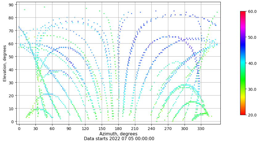
Azimuth-elevation plot for station ALC1. Signal to Noise S1C Data file ALC100ESP_R_2022186.xtr
