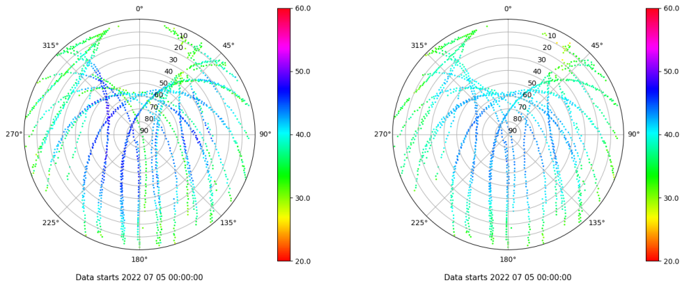
Skyplot for station ALC1. Signal to Noise S1C Data file ALC100ESP_R_2022186.xtr Skyplot for station ALC1. Signal to Noise S2C Data file ALC100ESP_R_2022186.xtr
